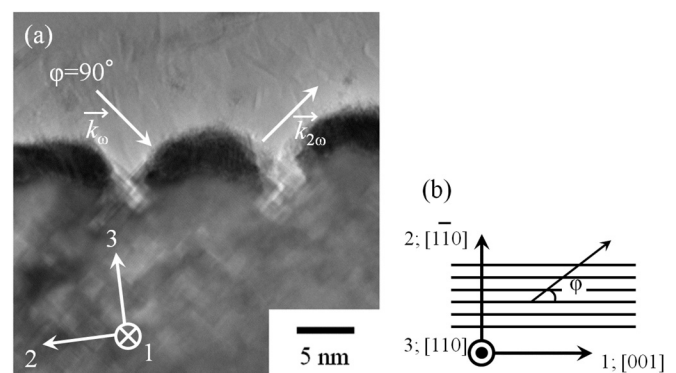
FIG. 3. (a) The cross-sectional shapes of the Pt nanowires on the MgO(110) faceted template observed by TEM. Two arrows show the wave vectors, \vec{k}_\omega and \vec{k}_{2\omega} , of the fundamental and SHG light beams for \varphi = 90^\circ , respectively. (b) The rotation angle, \varphi , defined as the angle between the plane of incidence and the direction 1; [001]; on the MgO (110) template.
