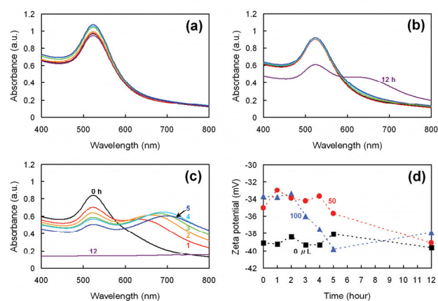
Fig. 3 Time dependence of absorption spectra of the Au NP dispersions containing (a) 0, (b) 50 and (c) 100 \mu\text{L} of \text{CaCl}_2 solution. Black, red, orange, green, light blue, blue, and purple lines represent 0, 1, 2, 3, 4, 5, and 12 h incubation periods, respectively. (d) Time dependence of the ZP of Au NP dispersions containing 0 (black), 50 (red) and 100 \mu\text{L} (blue) of \text{CaCl}_2 solution.
