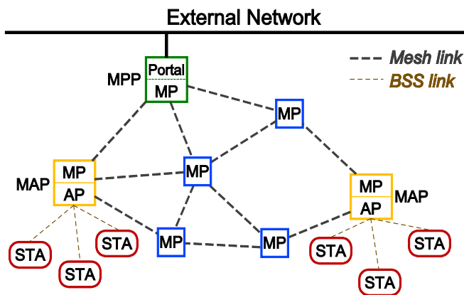
Figure 1. A basic architecture of WMN.
