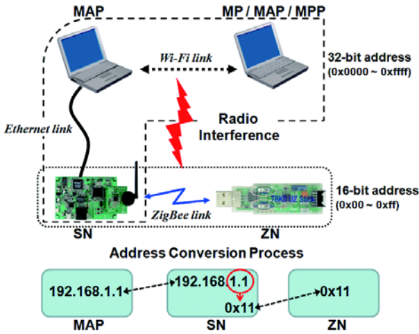
Figure 6. The interoperability issues in heterogeneous wireless networks: radio interference and addressing.
