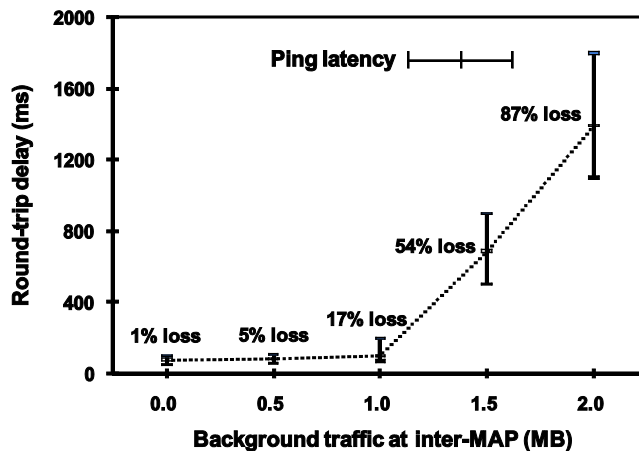
Figure 10. Effect of background traffic at inter-MAP on round-trip delay and packet loss.
