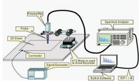
Fig. 2. Experiment layout.
