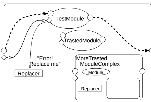
図 3.4: An Error Occured at Test Module
