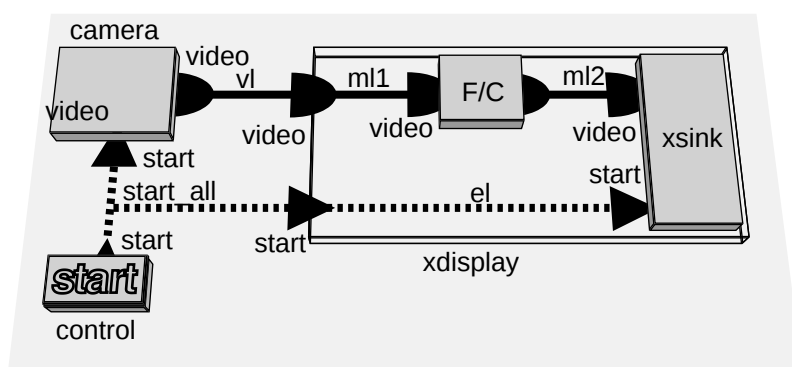
図 3.3: Our Application Structure
