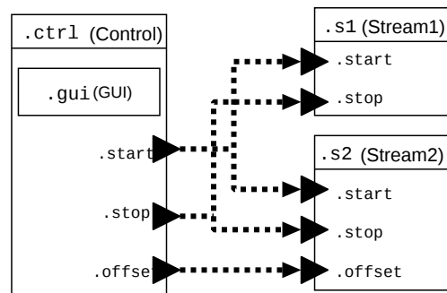
⊗ 5.5: Example of Module Scripting
