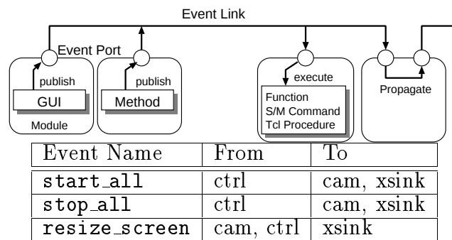
図 3.2: An Example of the Event Database
