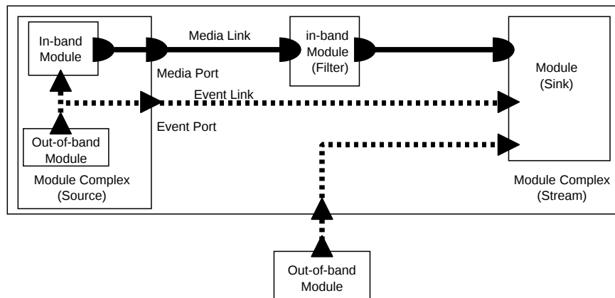
図 4.4: Rtm Application Development Environment
