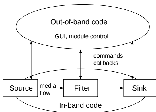
図 2.1: The Structure of Continuous Media Application
