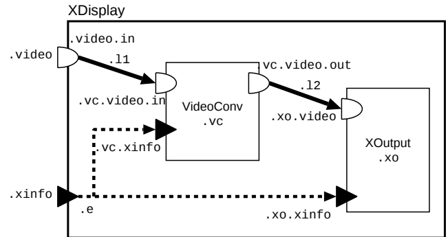
⊗ 5.4: Example of Module Scripting
