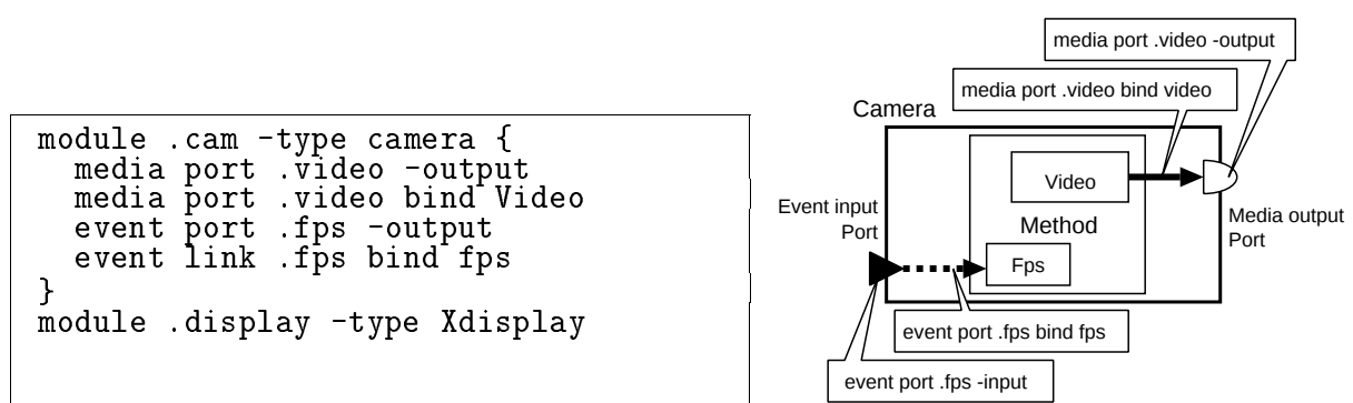
図 5.2: Example of Module Scripting
