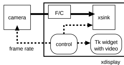
図 2.2: Former Application Structure
