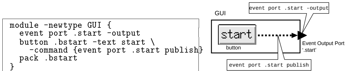
図 5.3: Example of Out-of-band Module Scripting
