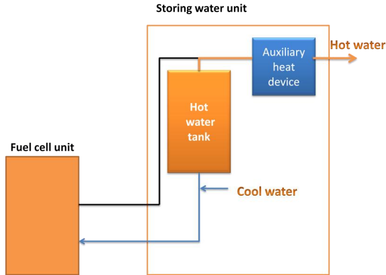
Figure 3.8: Supplying water behavior
