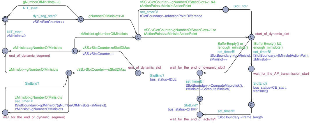
Figure 3.15: MAC dynamic segment model in UPPAAL
