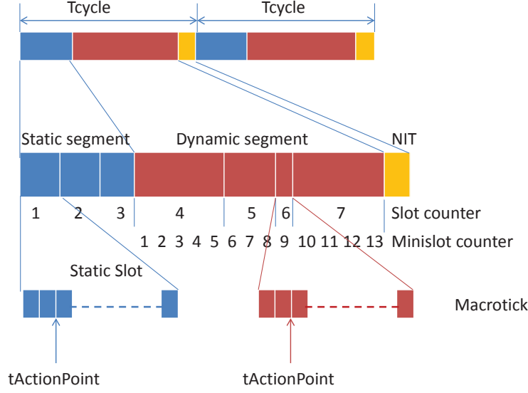
Figure 3.5: Communication cycle of FlexRay model
