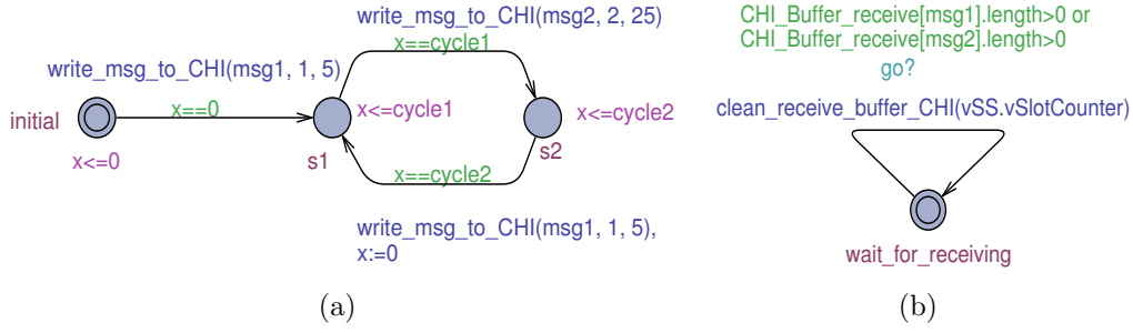
Figure 4.2: (a) The sender model and (b) the receiver model in UPPAAL
