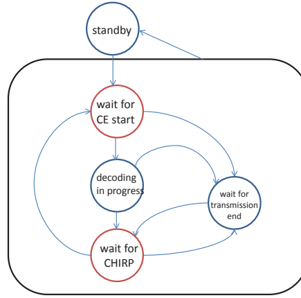
Figure 3.19: Overview of frame and symbol processing
