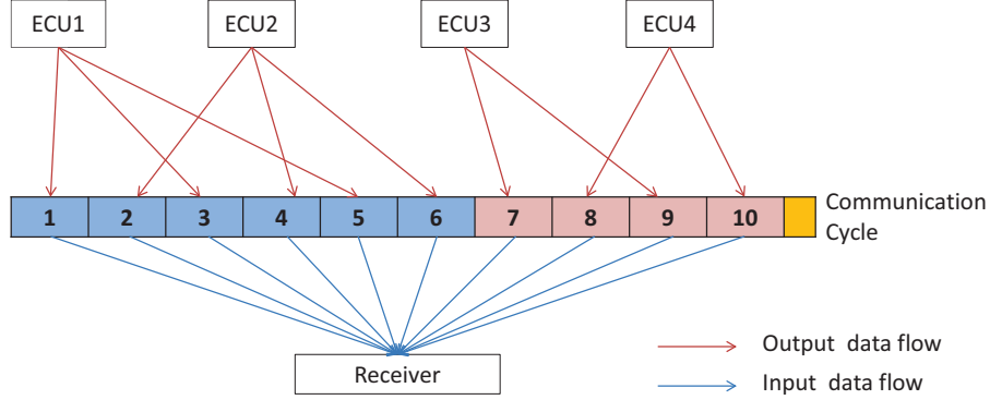
Figure 5.1: Testing example model in UPPAAL
