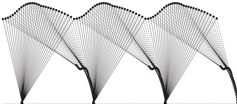
Fig. 15. Stick diagram for steady skipping gait.
