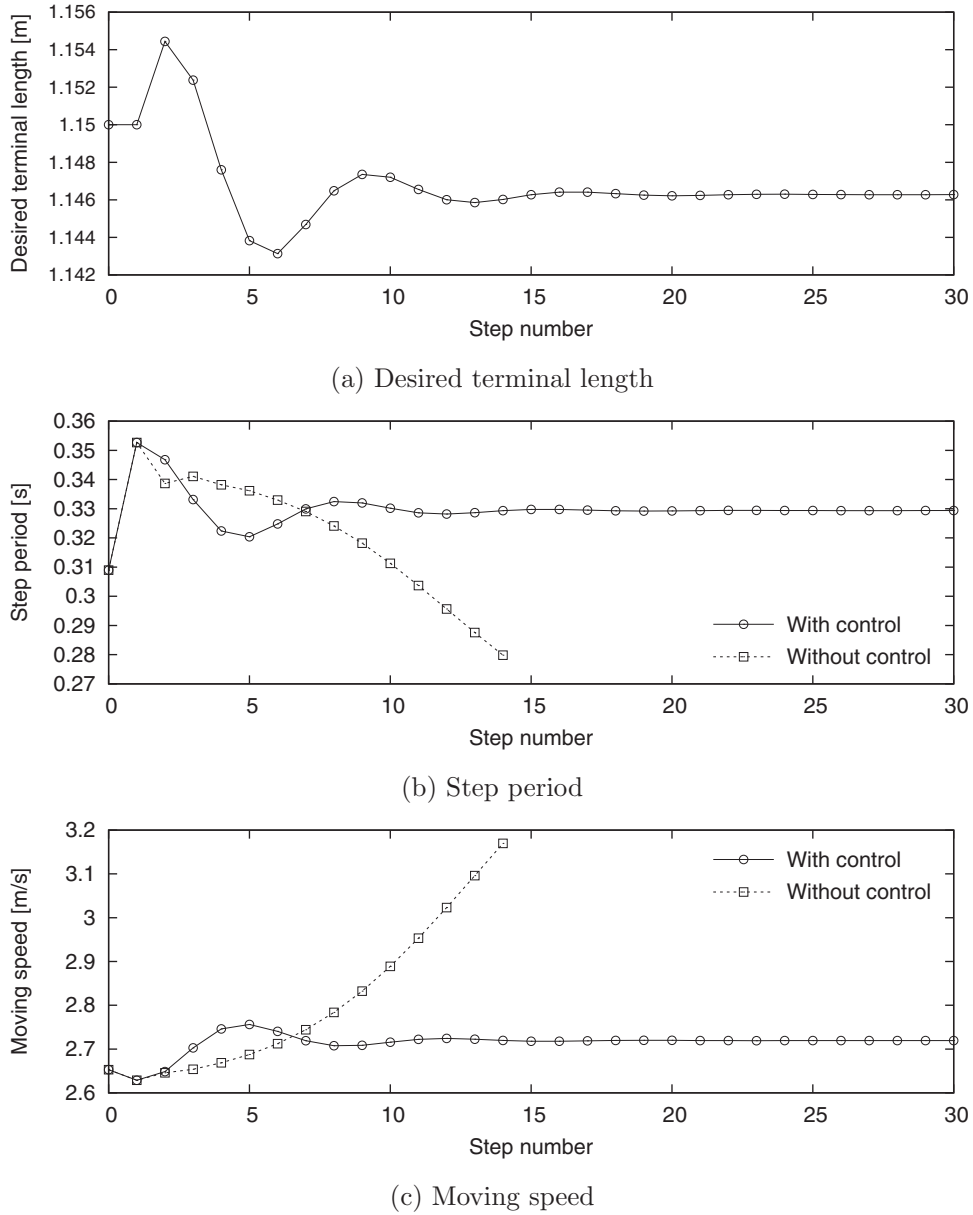
Fig. 8. Convergence of gait descriptors. (a) Desired terminal length; (b) step period; (c) moving speed.
