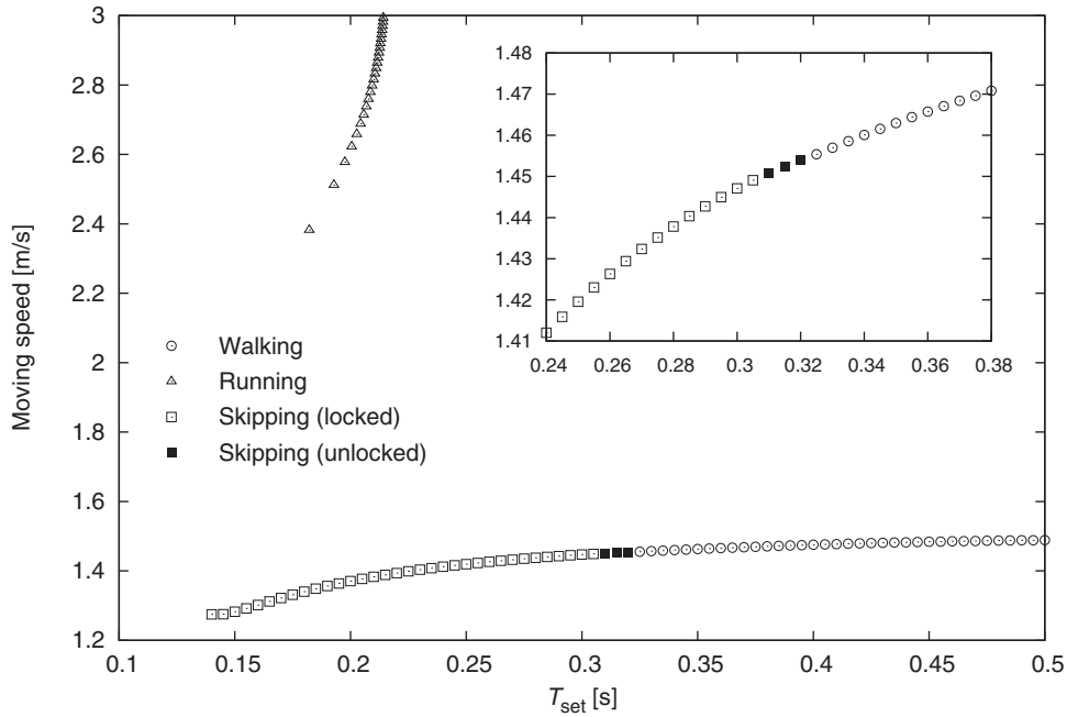
Fig. 17. Moving speeds as function of T_{\text{set}} .
