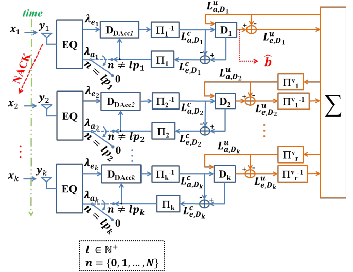
Fig. 2. Receiver of doped-accumulator assisted turbo HARQ systems
