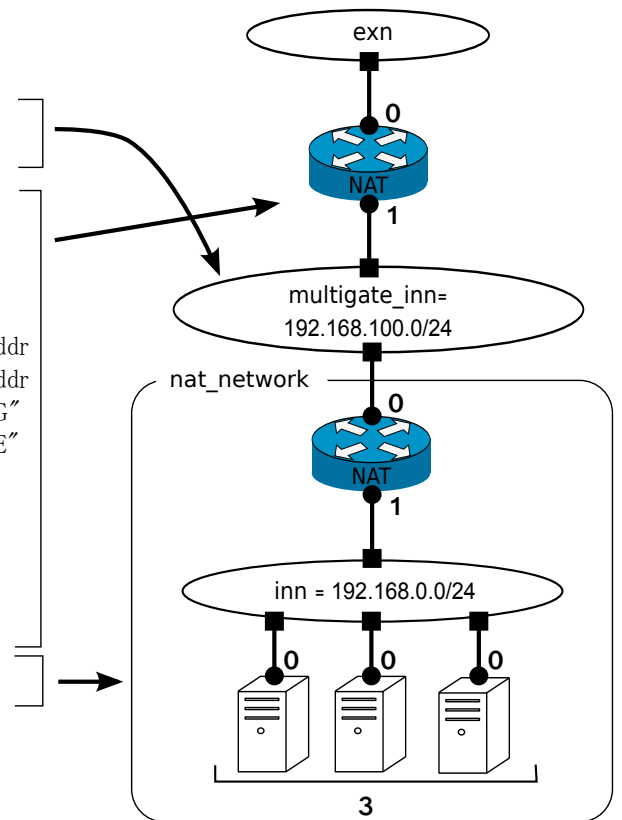
图 4.12: Multigate_NAT Dodule script
