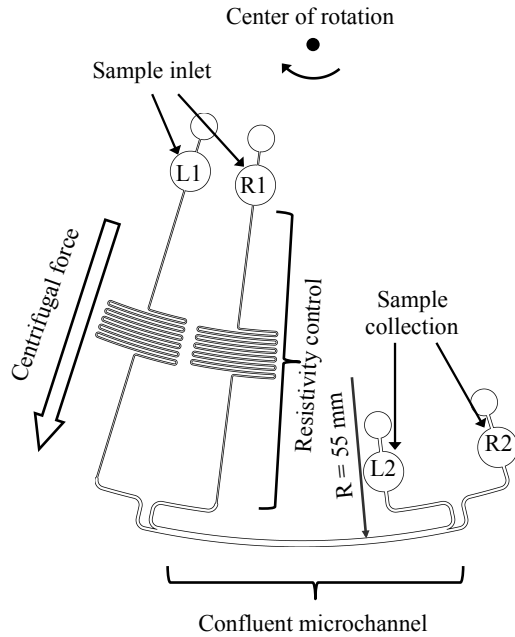
Fig. 5 Schematic illustration of microfluidic channels.
