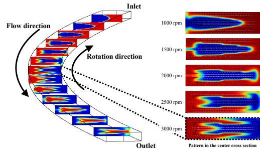
Fig. 7 Simulated secondary flow behavior.
