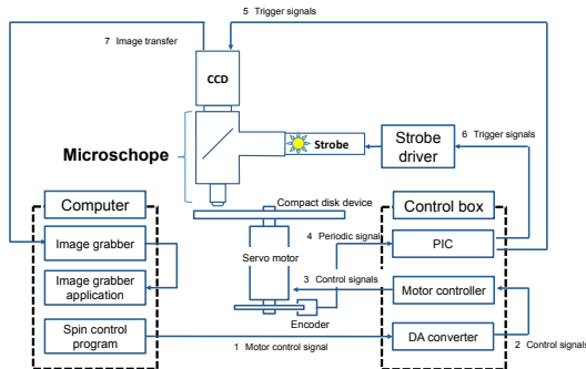
Fig. 2 Schematic illustration of micro strobe scope.
