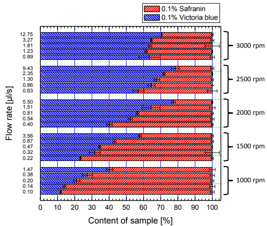
Fig. 8 Effect of spinning speed and flow rate on the magnitude of mixing.
