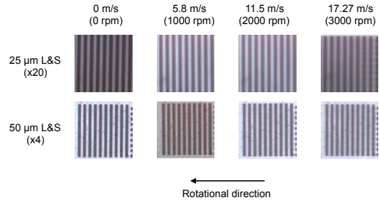
Fig. 3 Observed test patterns using microstrobe scope.
