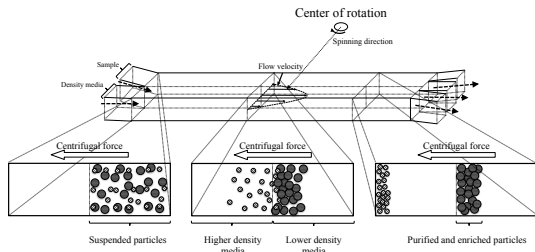
Fig. 1 Schematic illustration of continuous density gradient centrifugation.
