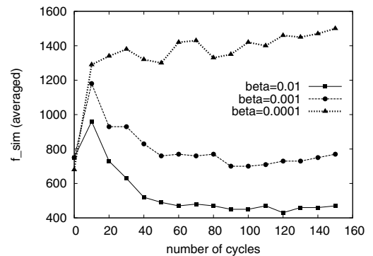
Fig. 5. Averaged transition of f_{sim} , with \beta = 0.01, 0.001, 0.0001
