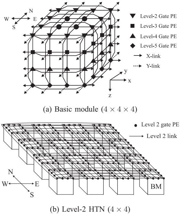
Figure 1. Interconnection of a HTN
