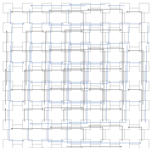
Figure 6. Perfect-shuffle traffic patterns on a 8 \times 8 mesh network
