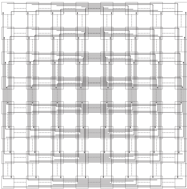
Figure 4. Center-reflection traffic patterns on a 8 \times 8 mesh network
