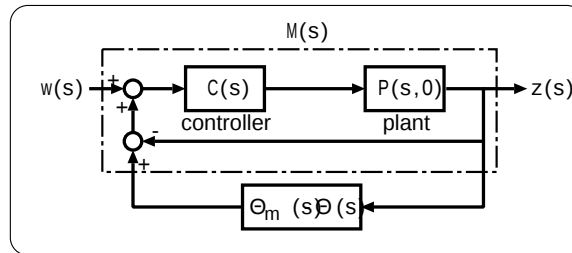
図 4.4: Uncertainty-Nominal loop for Smith method.
