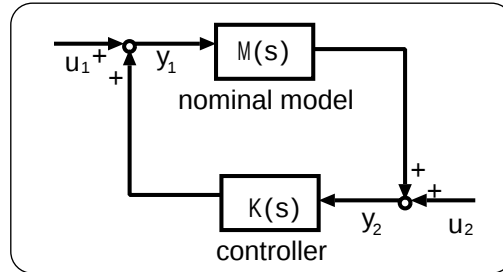
図 2.1: Internal stability analysis diagram.
