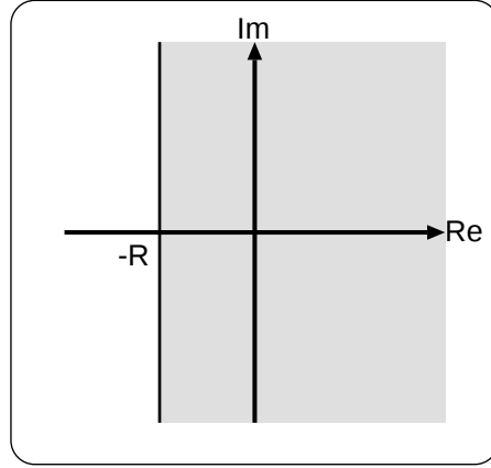
図 5.5: location of the zeros of (5.26)equation.
