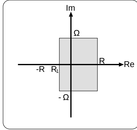
図 5.7: location of the zeros in a low frequency.
