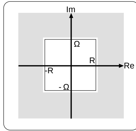
図 5.2: location of the zeros of (5.2)equation.
