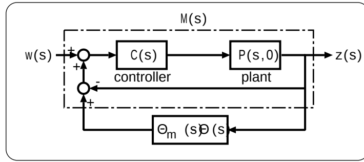
図 6.1: Uncertainty-Nominal loop for Smith method.
