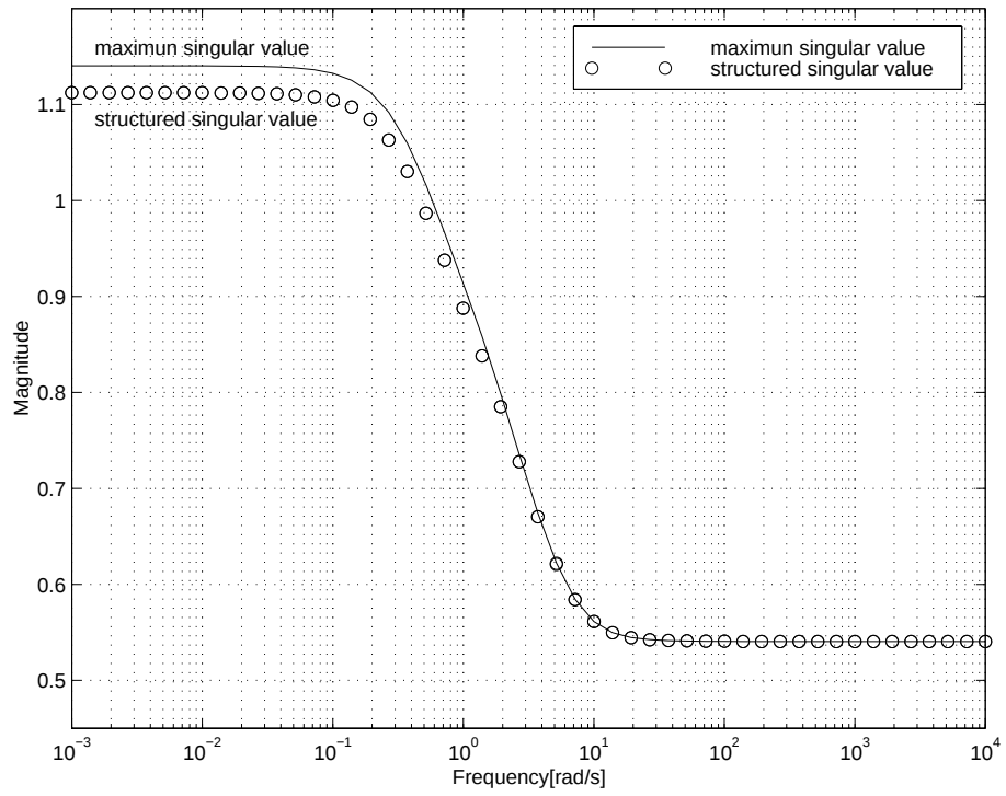
Fig 6.4: \mu_{\Delta}(M(j\omega)) and \bar{\sigma}(M(j\omega)) .
