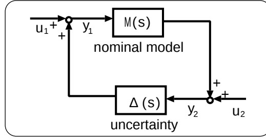
図 2.2: loop for stability analysis.
