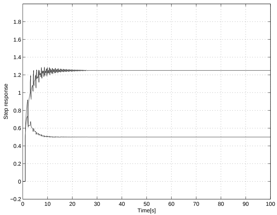
Fig 6.3: step response.
