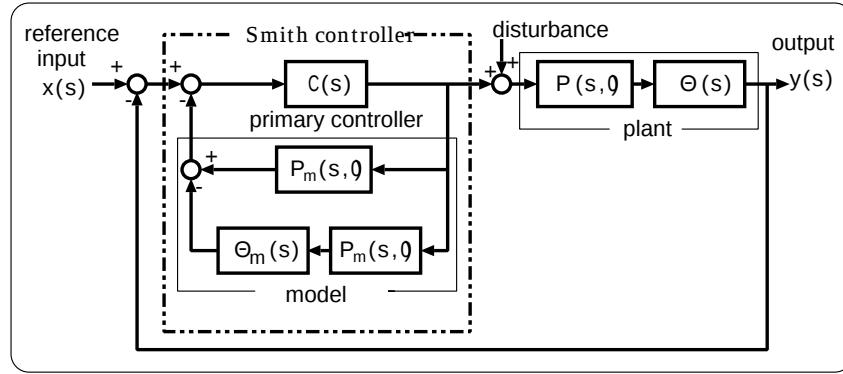
図 4.3: MIMO Smith method for decomposition plants.
