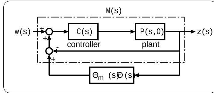
図 5.1: Uncertainty-Nominal loop for Smith method.
