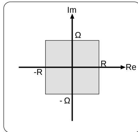
図 5.3: location of the zeros of (5.3)equation.
