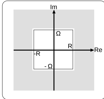
図 5.4: location of the zeros of (5.24) equation.
