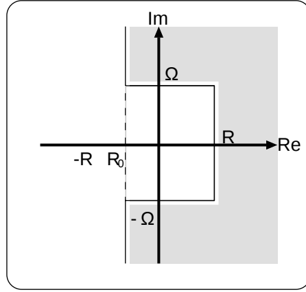
図 5.6: location of the zeros of (5.27)equation.
