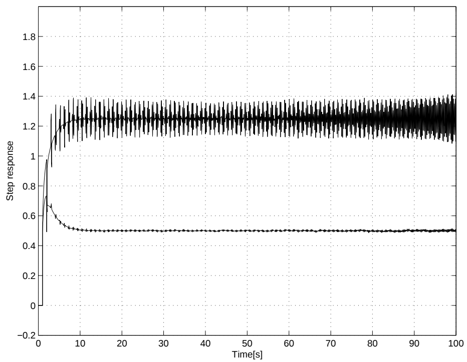
Fig 6.5: step response.
