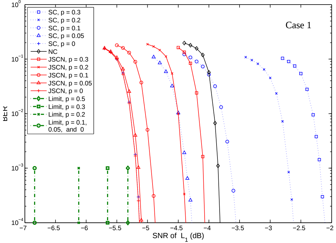
Figure 5.9: BER performance of the proposed JSCN technique for MARC with correlated sources in Case 1, with respect to the SNR of L_1 . Different source correlation are considered.
