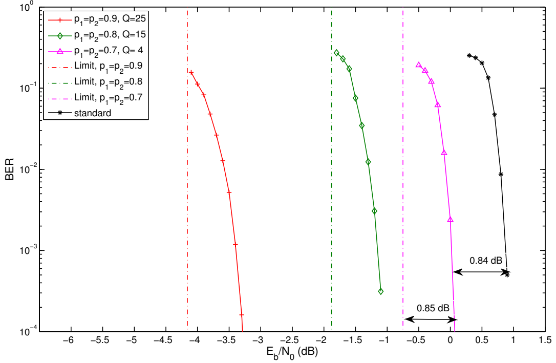
Figure 3.9: BER performance of the proposed technique for symmetric binary Markov sources in AWGN channels. Code rate is 1/2 .
