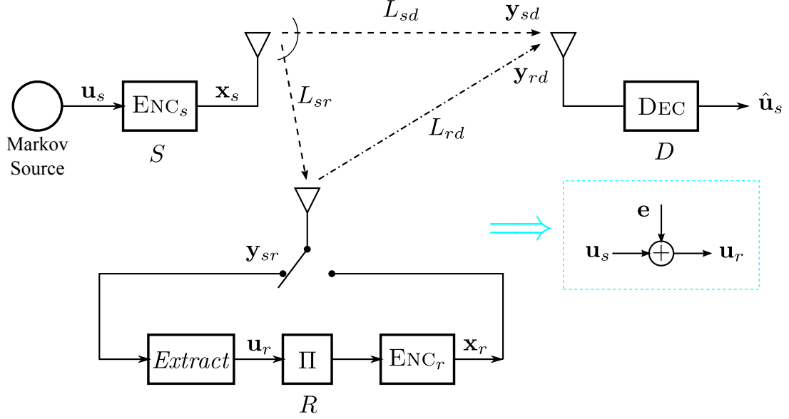
Figure 4.1: Block diagram of the binary Markov source transmission in a one-way relay system and its equivalent bit-flipping model. S , R and D denote the source, relay and destination node, respectively.
