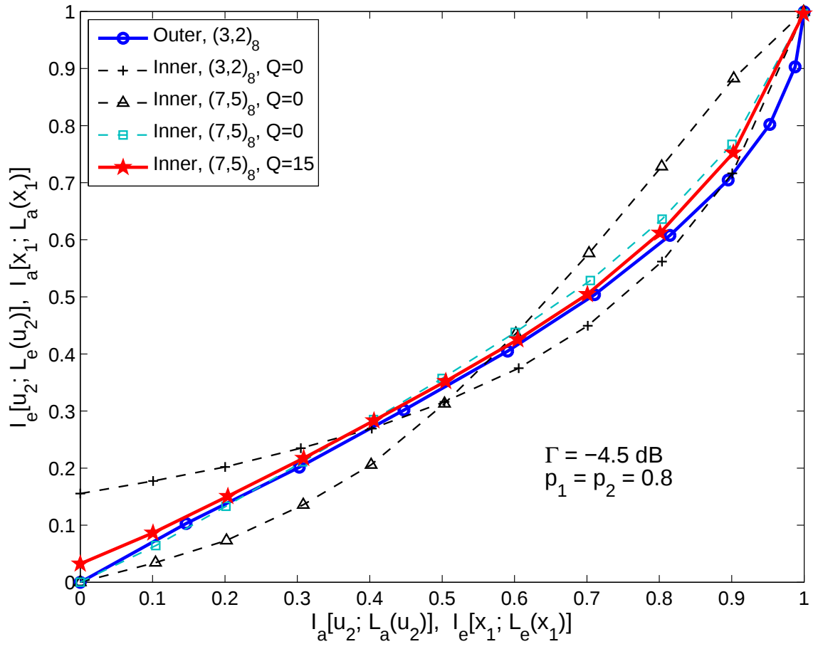
Figure 3.7: An example of determining optimal inner code and doping rate for Markov source with p_1 = p_2 = 0.8 .
