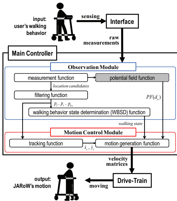
Fig. 3. Data/control flow for the JARoW controller system (Details of the potential field function can be found in [9].)
