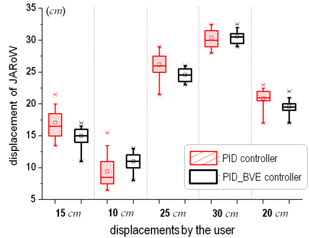
Fig. 6. Comparison of JARoW's displacements based on the PID controller in [9] and the PID_BVE controller, respectively, for different stride lengths
