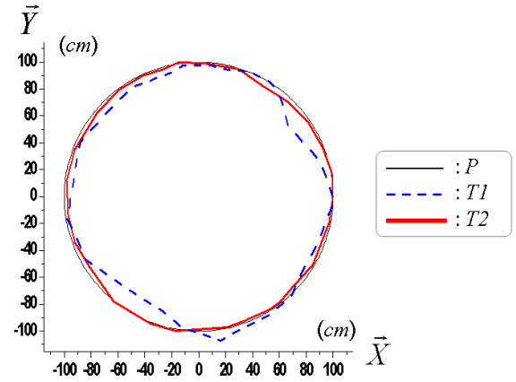
Fig. 5. Trajectories of JARoW following a circular path (thin black line), where the blue dashed line and the red solid line indicate trajectories obtained using the controller in [8] and the proposed controller, respectively
