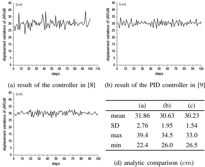
Fig. 4. Comparison of JARoW's displacement variations for uniform stride lengths of 30cm
