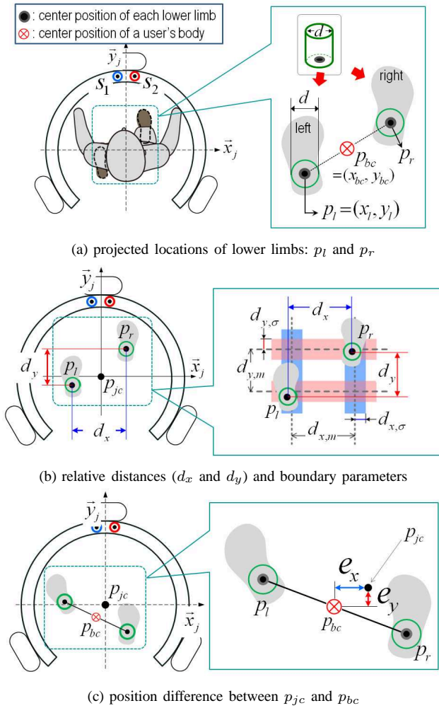
Fig. 2. Illustrations of definitions and notations used in the walking intent based movement control
