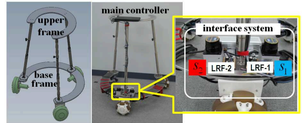
Fig. 1. Prototype of JARoW and its user interface system
