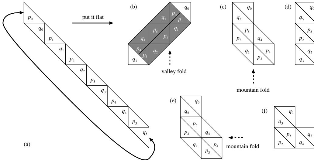
Figure 2: Piano-hinged loop with n = 3 (a), and two sequences of folding operations that result in a doubly covered straight tromino (b, c, d) or L tromino (b, e, f). Gray denotes the back side of the pieces.
