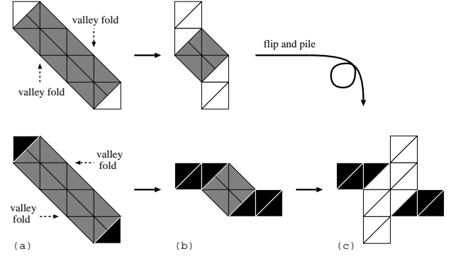
Figure 4: Crossover gadget
