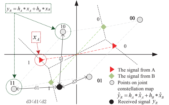
Fig. 3. A sends x_A = '1' , which is the red triangle marked by a red dotted circle. The overlapped signals that A expects to receive are the gray points marked by the green dotted circles. The received signal is presented with the black point. Even when the distances d1, d2, d3 satisfy d3 < d1 < d2 , the receiver A will demodulate the signal to '11'.
