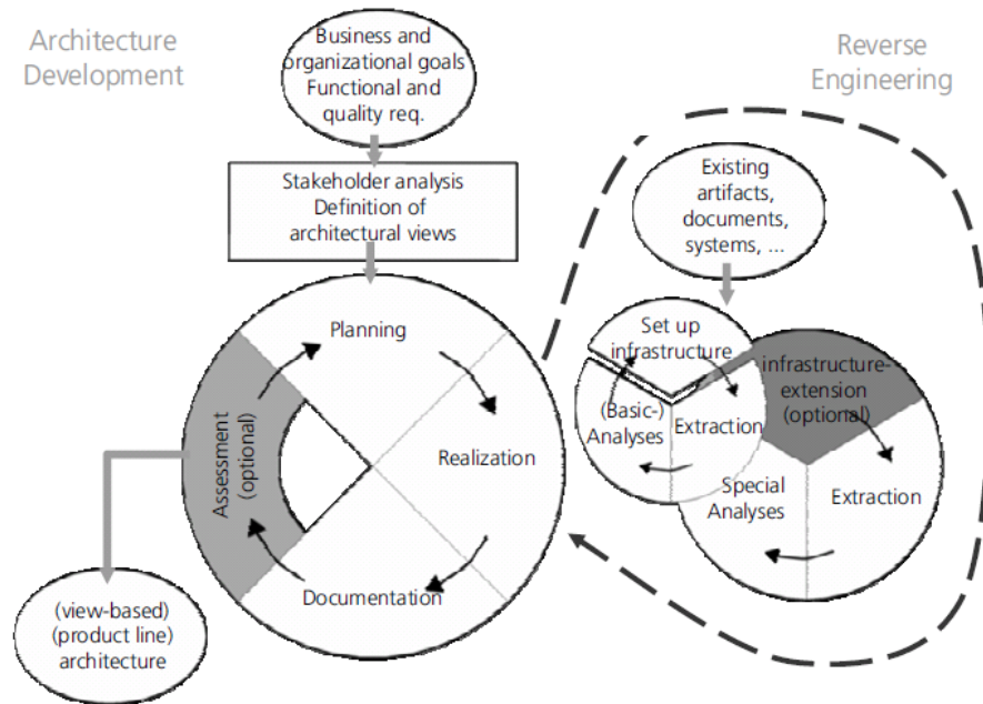
Figure 40 Pulse-DSSA Process
