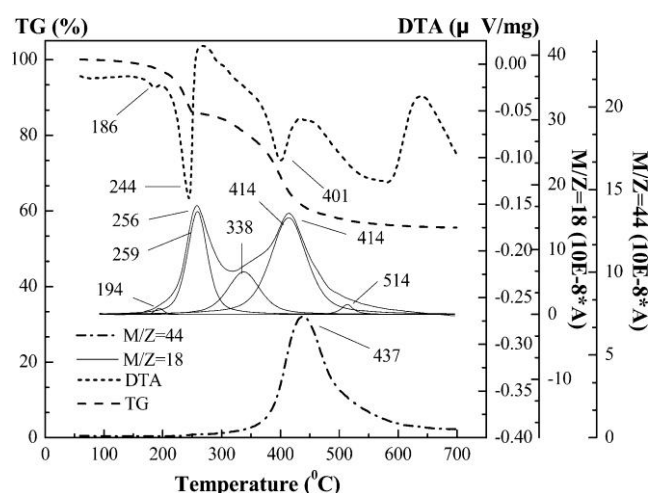
Figure 3 TG-DTA-MS curves of hydrotalcite ( \text{Mg}_3\text{Al-CO}_3 HT). [Reproduced with permission from American Chemical Society (ACS) of ref. 10]
