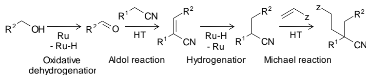
Scheme 8 Tandem reaction catalyzed by \text{Ru}/\text{hydrotalcite}
