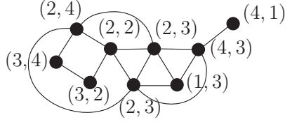
Figure 2: An example of UNO-1 graph.
