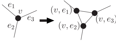
Figure 3: A node gadget splits a vertex into three vertices to form a triangle.
