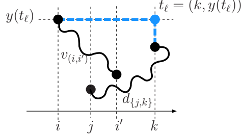
Figure 6: An example case of the DP.
