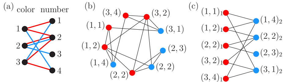
Figure 7: (a) UNO cards are edges of a bipartite graph, and they are partitioned into two subsets (red and blue) in UNO-2; (b) adjacency of UNO cards becomes a line graph of a bipartite graph; and (c) an UNO-2 graph is a bipartite graph by removing edges in each partite set.
