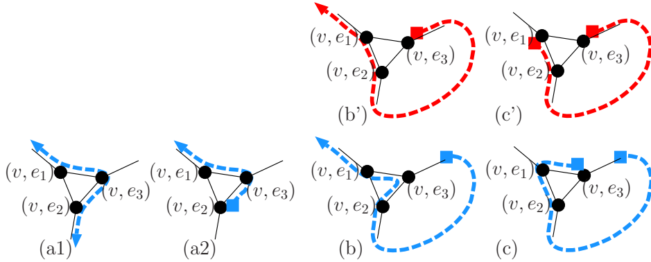
Figure 4: Possible tours passing through a node gadget. Each dotted line is a part of a tour, and a square denotes either end of a tour.
