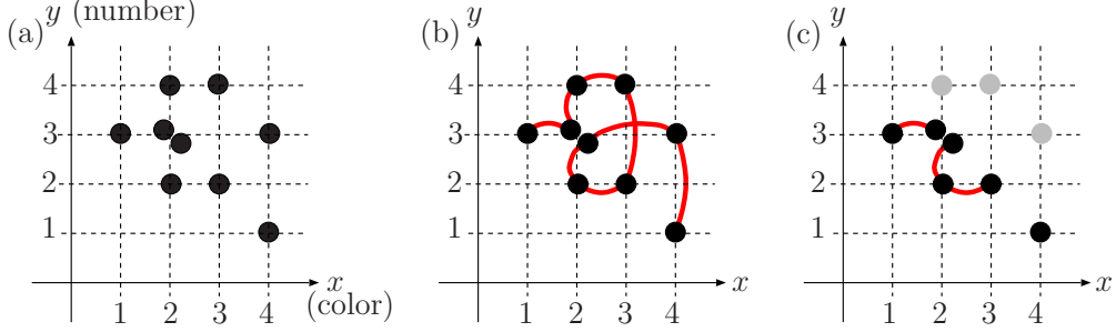
Figure 5: (a) Geometric view of an UNO-1 graph, where all the edges are omitted, (b) a Hamiltonian path in the UNO-1 graph, and (c) a set of subpaths in the subgraph of the UNO-1 graph induced by the first six points; it shows h_{\{1,2\}} = 1 , v_{(2,3)} = 1 and d_{\{4,4\}} = 1 .
