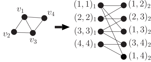
Figure 1: Reduction from HP to UNO-2.
