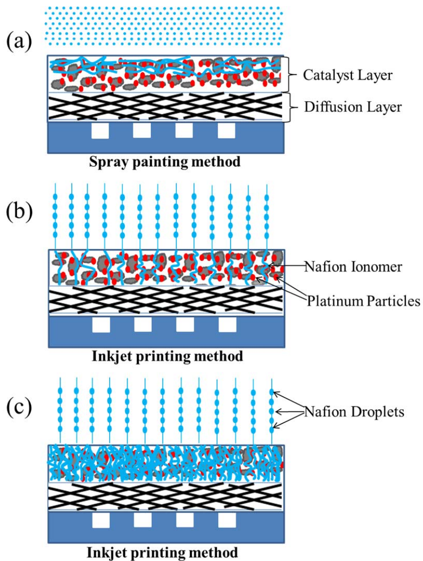
Fig. 6 Schematic views of the cross-section of the catalyst layer. Red shows Pt particles. Blue shows Nafion ionomer. Black shows carbon aggregates. (a) Low Nafion content using spray painting for which not all catalyst particles are connected to the membrane by Nafion ionomer. (b) Appropriate loading of the Nafion ionomer condition using inkjet printing. (c) Mass volume of Nafion loading condition using inkjet printing.
