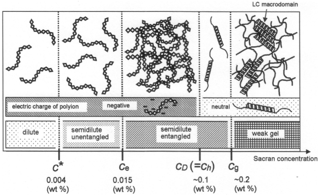
FIG. 11. Schematic illustrations representing the chain conformation of sacran in salt-free solutions [( c^* ) overlap concentration, ( c_e ) entanglement concentration, ( c_D ) critical polyelectrolyte solution, ( c_h ) helix transition concentration, ( c_g ) gelation concentration].
