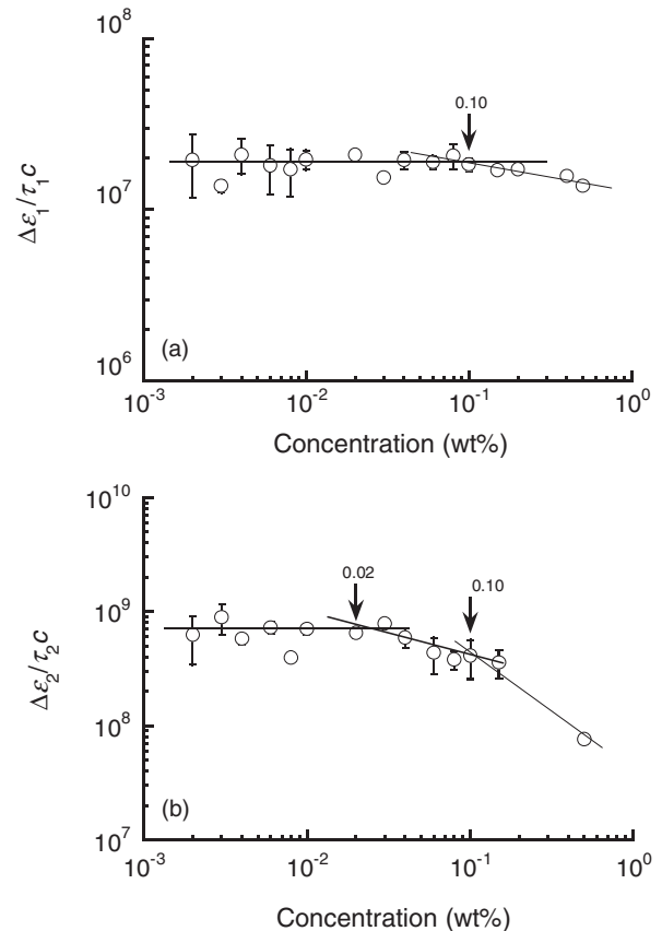
FIG. 10. \Delta\varepsilon/\tau c for (a) strongly bound counterions and (b) loosely bound counterions for sacran solutions as a function of sacran concentration.
