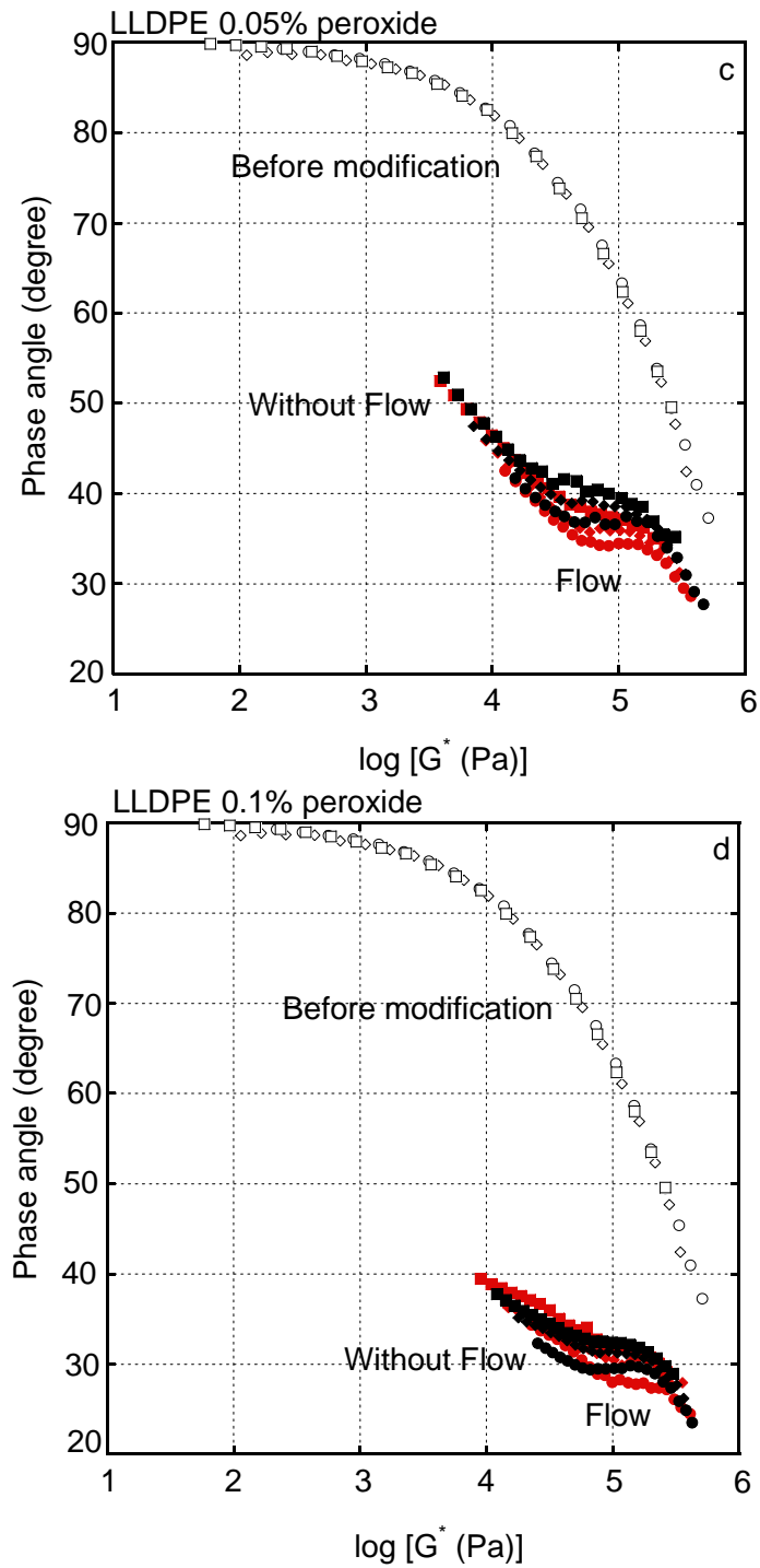
Figure 2-19. van Gurp-Palmen plots for samples (open symbols) before modification and after modification (closed symbols) under flow field and (red symbols) without flow field; at (circles) 130 °C, (diamonds) 160 °C and (squares) 190 °C; (a) LDPE 0.05 wt.%, (b) LDPE 0.1wt.%, (c) LLDPE 0.05 wt.% and (d) LLDPE 0.1 wt.% peroxide.
