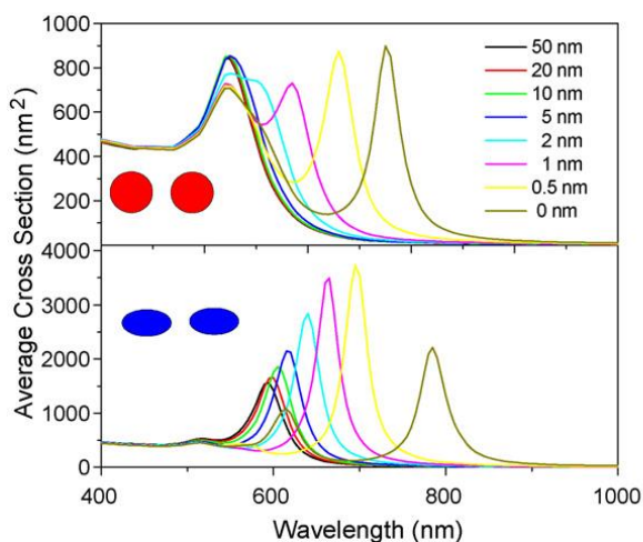
Figure 1.4. Red shift of the extinction cross-section of a pair of 20 nm gold spheres (upper panel) and ellipsoids with aspect ratio 2 (lower panel) as the separation distance between them is reduced (calculations based on the boundary element method). 55
