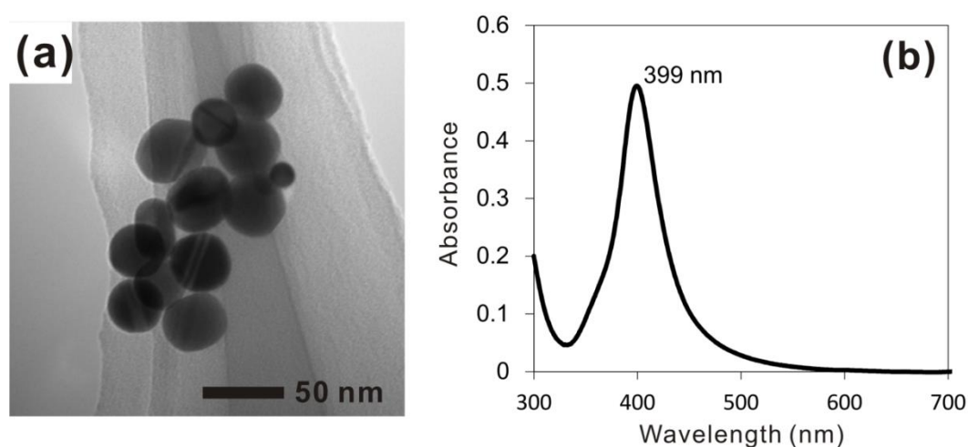
Figure 3.2. (a) TEM image of as-synthesized Ag nanoparticles capped with the citrate molecule, (b) UV-Vis spectrum of as-synthesized Ag nanoparticles with peak maximum of 399 nm.
