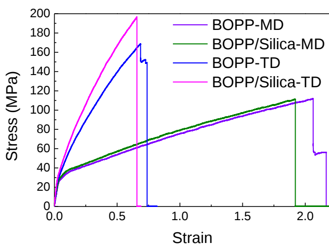
Figure 7. Strain-stress curves of BOPP and BOPP/Silica.
