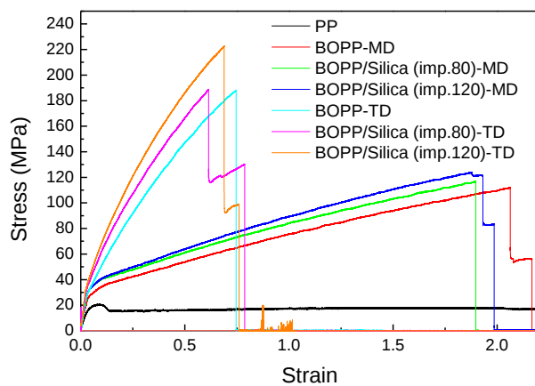
Figure 13. Stress-strain curves of BOPP/Silica with different silica content.
