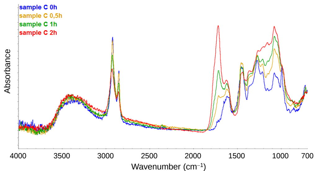
Figure 3. ATR-IR spectra of (a) sample A, (b) sample B and (c) sample C.
