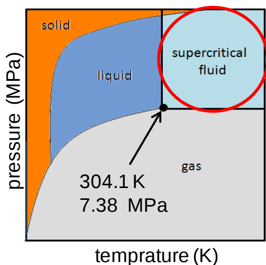
Figure 20. Schematic phase diagram for a pure \text{CO}_2 .
