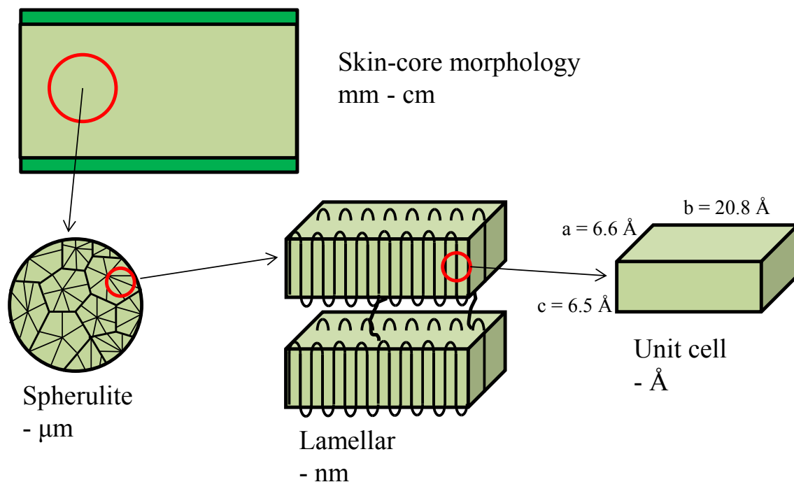
Figure 3. Higher order structure of PP.
