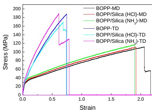
Figure 12. Stress-strain curves of BOPP/Silica prepared with different catalyst.
