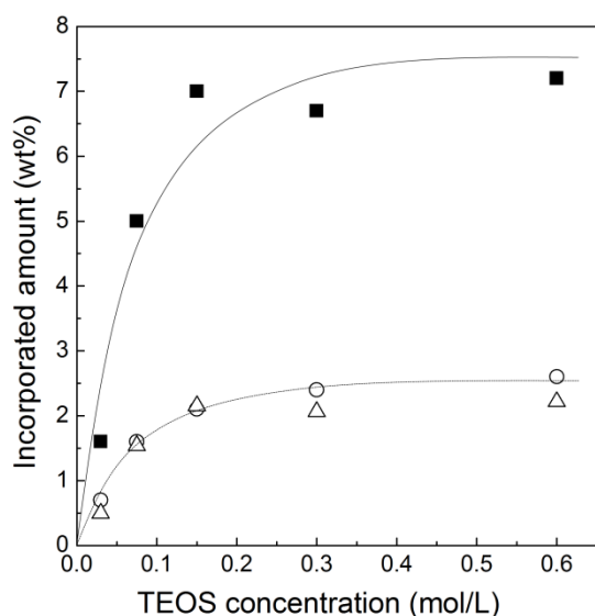
Figure 1. Effect of the TEOS concentration on incorporated amounts : (■) TEOS, (○) silica, and (Δ) the theoretical silica content.
