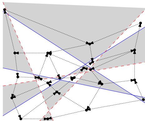
Fig. 10: Orientation of the dual graph G of a bichromatic line arrangement. Cells of b-out-colored vertices are drawn as shaded, while cells of r-out-colored vertices are drawn white. Every bichromatic vertex of the arrangement yields a four-cycle in the oriented graph.
