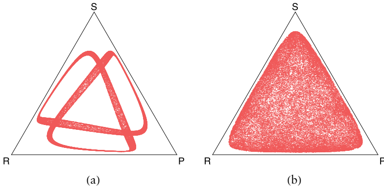
Figure 1. The (a) quasiperiodic tori and (b) chaos in the phase space of the continuous-time limit model with parameters a = 0 , b = 1 , \epsilon_1 = -\epsilon_2 = 0.5 , and two different initial conditions.
