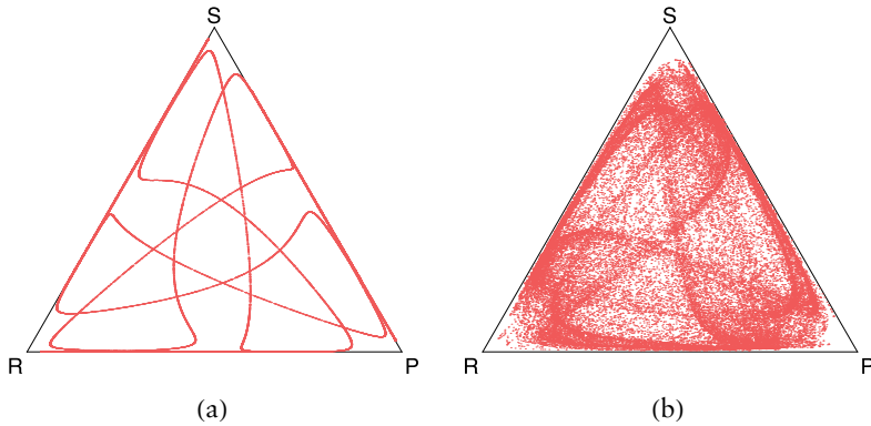
Figure 2. A limit cycle ((a): \epsilon_2 = 0.025 ) and chaotic trajectory ((b): \epsilon_2 = -0.365 ) in the phase space of the continuous-time limit model with parameters a = 0.01 , b = 1 , \epsilon_1 = 0.5 , and random initial conditions.
