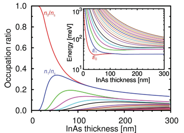
FIG. 3. The electron occupation ratio n_i/n_s (from above i = 0, 1, 2, \dots ), where n_s and n_i are the total and the i -th subband sheet concentration, respectively. Inset: the calculated quantized electron energy levels E_i (from below i = 0, 1, 2, \dots ), measured from the surface conduction band bottom.
