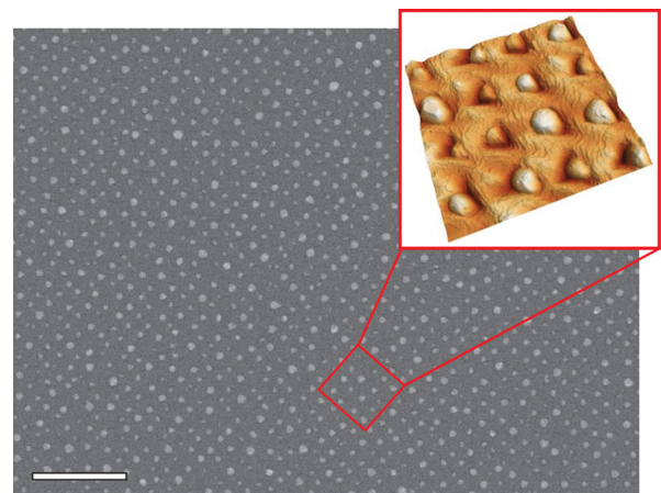
FIG. 2. SEM image of the self-organized growth of Au-Si islands on Si(111) surface patterned with an array of holes. Scale bar is 200 nm and distance between islands is 80 nm. Inset is a 3D STM image showing a regular arrangement of 4 \times 4 islands.
