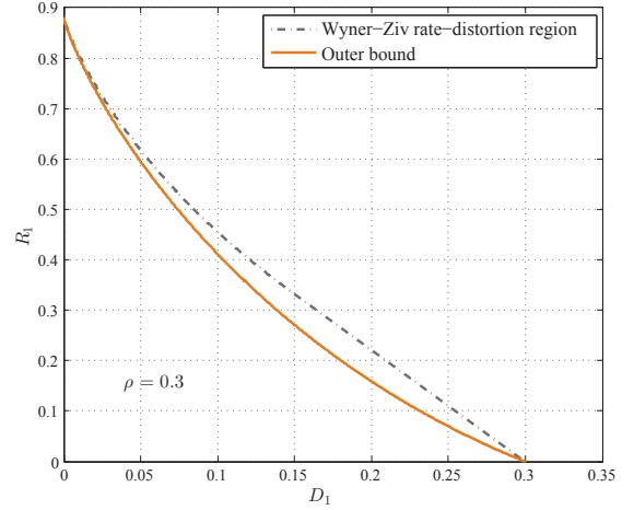
Fig. 5. The comparison of Wyner-Ziv rate-distortion region and derived outer bound. The correlation \rho between two sources is set at 0.3.
