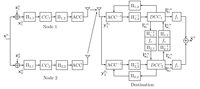
Fig. 7. Block diagram of the encoding/decoding algorithm shown in [10] and [16].
