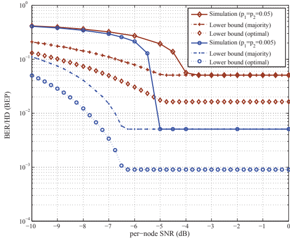
Fig. 8. Symmetric P and SNR. BPSK is used for both nodes.
