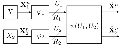
Fig. 3. The binary multiterminal source coding problem for two correlated binary sources.
