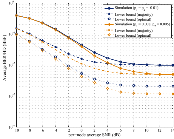
Fig. 12. Asymmetric SNR and P . BPSK is used for both nodes. Channels are assumed to suffer from block Rayleigh fading.
