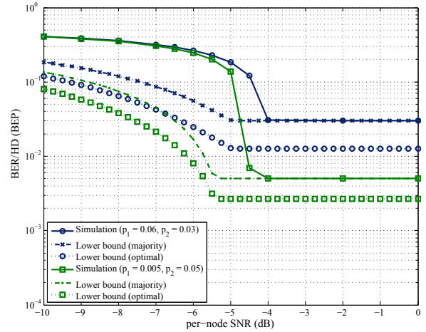
Fig. 9. Asymmetric P and symmetric SNR. BPSK is used for both nodes.
