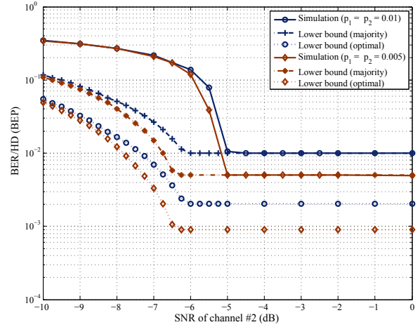
Fig. 11. Asymmetric r_1 and r_2 . The coding rates r_1 and r_2 are set at 1 and \frac{1}{2} , respectively. The transmit power of two nodes are the same. QPSK is used for node 1 and BPSK for node 2.
