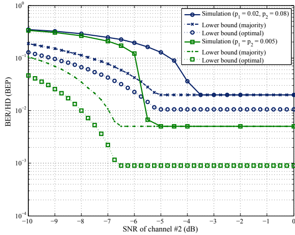
Fig. 10. Asymmetric r_1 and r_2 . The coding rates r_1 and r_2 are set at \frac{1}{4} and \frac{1}{2} , respectively. The transmit power of two nodes are the same. BPSK is used for both nodes.
