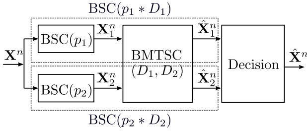
Fig. 6. The distortion model of the binary CEO problem. BMTSC represents binary multiterminal source coding.
