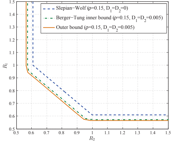
Fig. 4. The comparison of \mathcal{R}^o(D_1, D_2) , Berger-Tung inner bound and Slepian-Wolf admissible rate region. The correlation \rho between two sources is set at 0.15.
