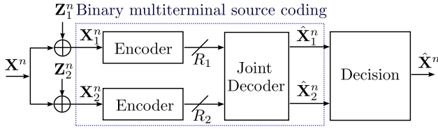
Fig. 2. The abstract model of the binary CEO problem with two independent nodes.
