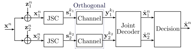
Fig. 1. The abstract system model of estimating a single source through two independent nodes with joint source-channel coding.
