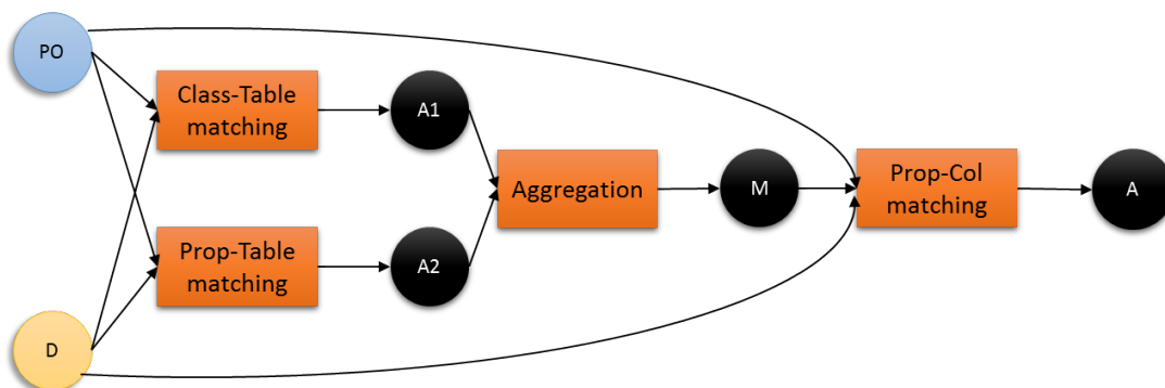
Figure 4.1: PivotOntology-Database matcher model
