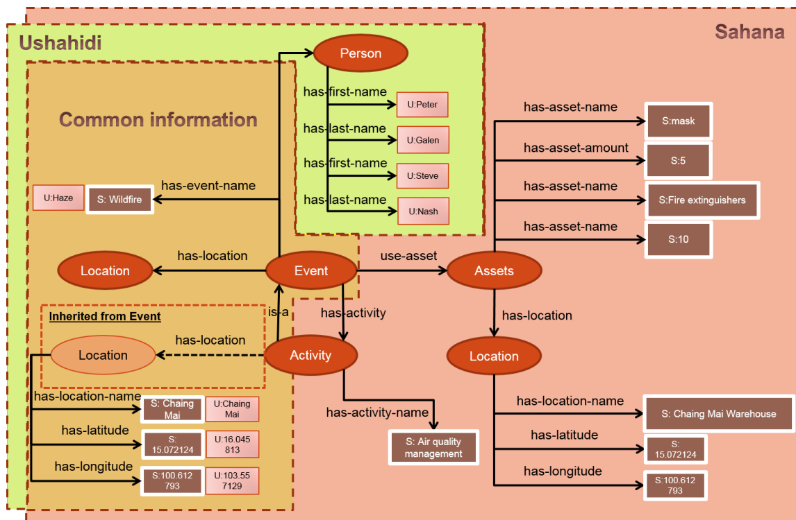
Figure 5.11: Information Sharing between Sahana and Ushahidi through HARE
