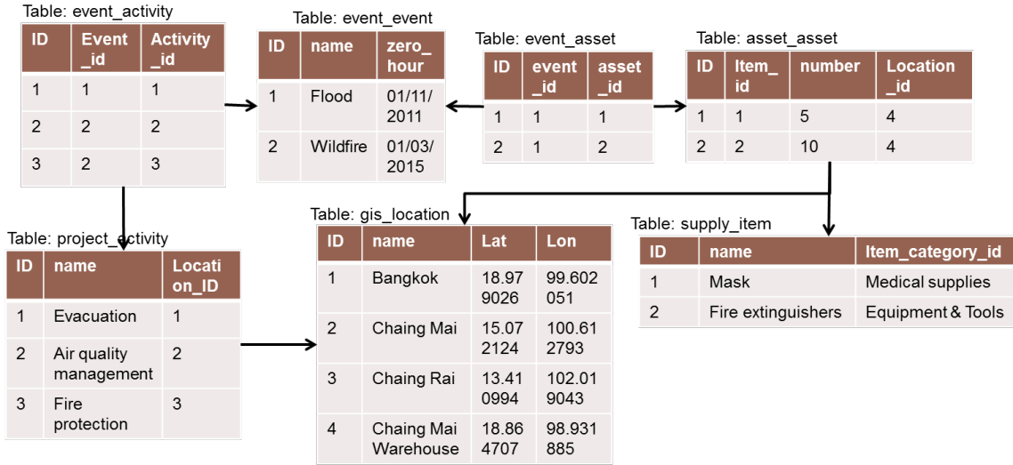
Figure 5.3: Example of Sahana schema
