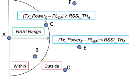
Fig. 1: Interference Model
