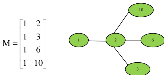
Fig. 3. Network example with its N and (N of N) plus matrix for vertex #1
