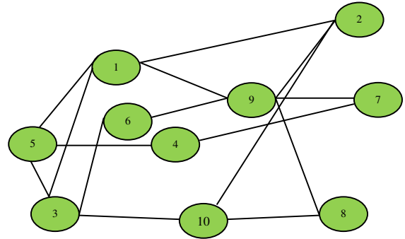
Fig. 1. Example of simple network
