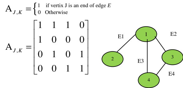
Fig. 2. The network graph and its incidence matrix
