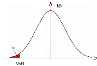
Fig. 1. The value at risk VaR and level \alpha = 1 - p
