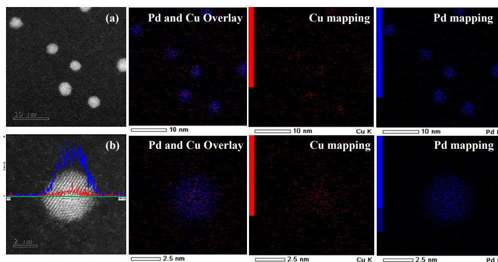
Figure 5. STEM-HADFF images and EDS-mapping results of \text{Pd}_{60}\text{Cu}_{40} -PVP NPs in different magnifications. The blue and the red line in image (b) was Pd and Cu distribution, respectively, determined by an EDS-line analysis on the green line.
