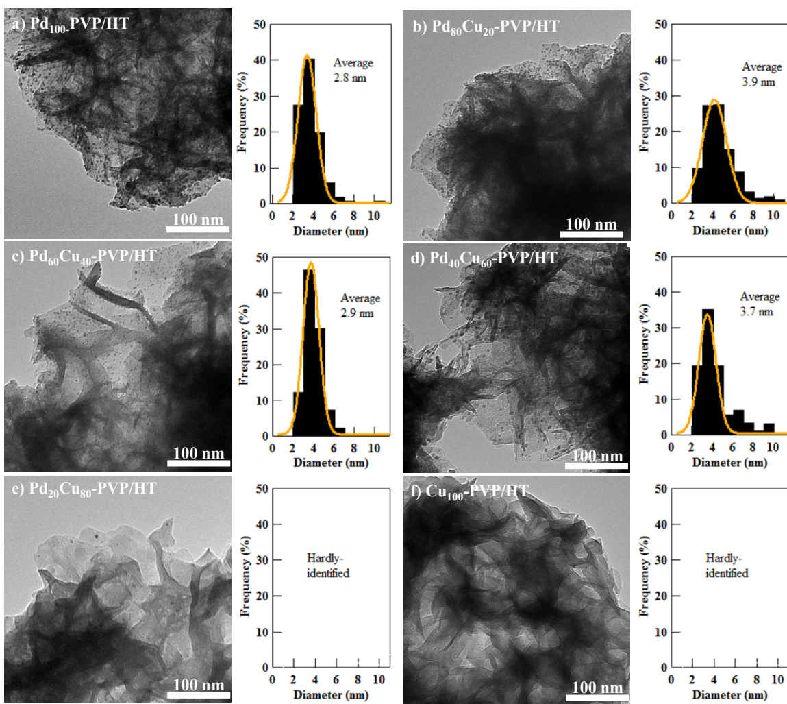
Figure 1. TEM images of Pd x Cu y -PVP/HT with particle size distributions.
