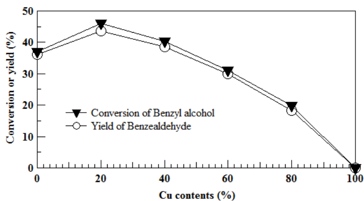
Figure 2. Activities for aerobic oxidation of benzyl alcohol toward benzaldehyde over Pd x Cu y -PVP/HT catalysts in toluene for 1 h at 313 K.
