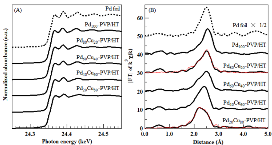
Figure 4. Pd K-edge XAS results in (A) XANES and (B) |FT| of k^3 -weighted EXAFS applied in the range of k = 3-15 \text{ \AA}^{-1} . The McKale fitting results are shown as the red dash lines in (B).
