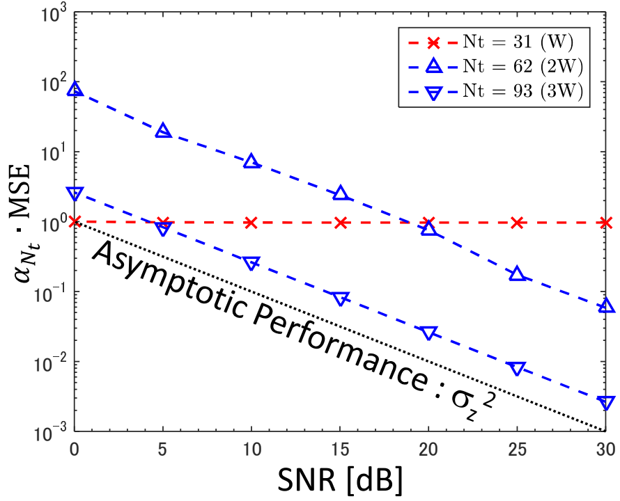
Fig. 1.3: The normalized performance of the LS estimator (1.6): \alpha_{N_t} \text{MSE} in the VA30 scenario, where the normalization factor \alpha_{N_t} denotes \alpha_{N_t} = N_t/W . The TS range without the GI (a) is assumed. The CIR length W is set at 31.
