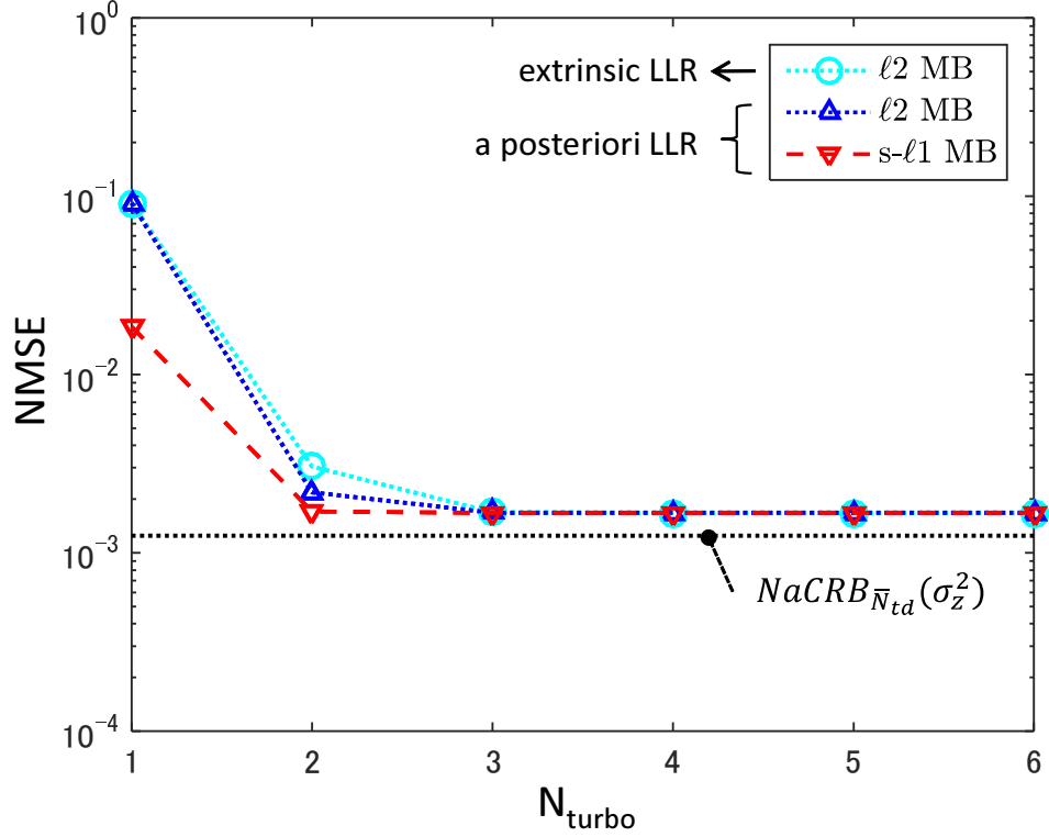
Fig. 3.7: NMSE convergence performance of the CHATES algorithms over turbo iterations. SNR is set at 15 dB. The VA30 scenario and Burst format 41 are assumed.
