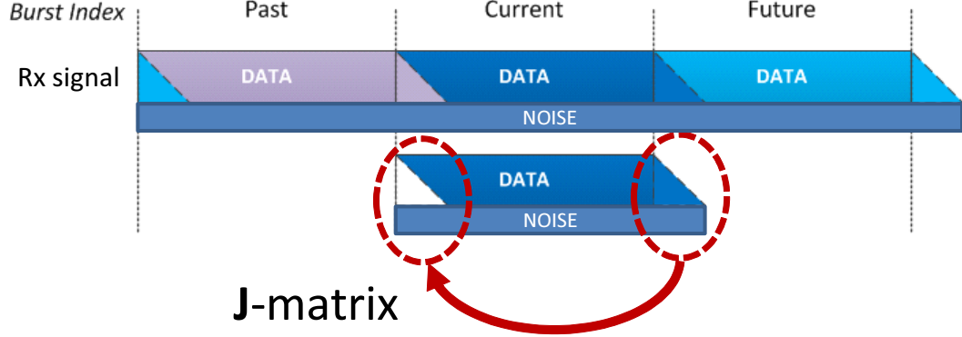
Fig. 3.1: Noise enhancement problem of CHATUE1 algorithm. Intuitively, the operation with J -matrix adds the leaked current signal to the future block onto the head part of the current signal, which causes the noise enhancement problem.
