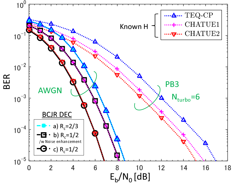
Fig. 3.4: BER performance in the 1-path static AWGN and in the PB3 scenario. The spectral efficiency is fixed to \eta = 0.4 . The CHATUE1 and CHATUE2 algorithms use Burst format 11 with the coding rate R_c = 1/2 , whereas TEQ-CP uses Burst format 12 with R_c = 2/3 . The known CIR H and six turbo iterations are assumed.
