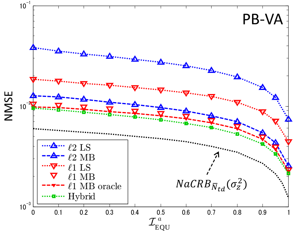
Fig. 2.14: NMSE convergence performance over the MI \mathcal{I}_{\text{EQU}}^a (2.49) in the PB-VA scenario at SNR is set at 15 dB.
