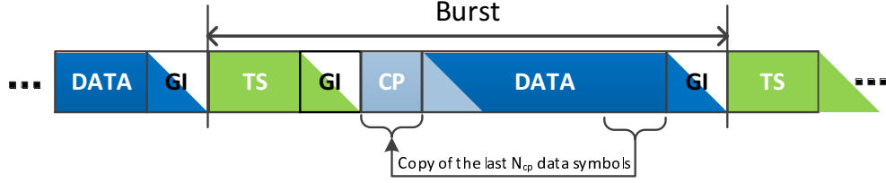
Fig. 1.1: An example of TX burst format. The triangle parts illustrate the IBIs.
