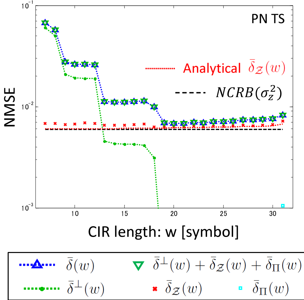
Fig. 2.22: The NMSE performance for possible CIR lengths w , where the PN TSs are used. \bar{\delta}(w) denotes the NMSE of the channel estimate \hat{\mathcal{H}}_{[w]}^{MB} . \bar{\delta}^{\perp}(w) , \bar{\delta}_{\mathcal{Z}}(w) and \bar{\delta}_{\Pi}(w) are normalized variances of (2.67), (2.68) and (2.69), respectively. The red dotted curve Analytical \bar{\delta}_{\mathcal{Z}}(w) is the NMSE normalized (2.70) with \mathbb{E}[\|\mathcal{H}\|^2] .
