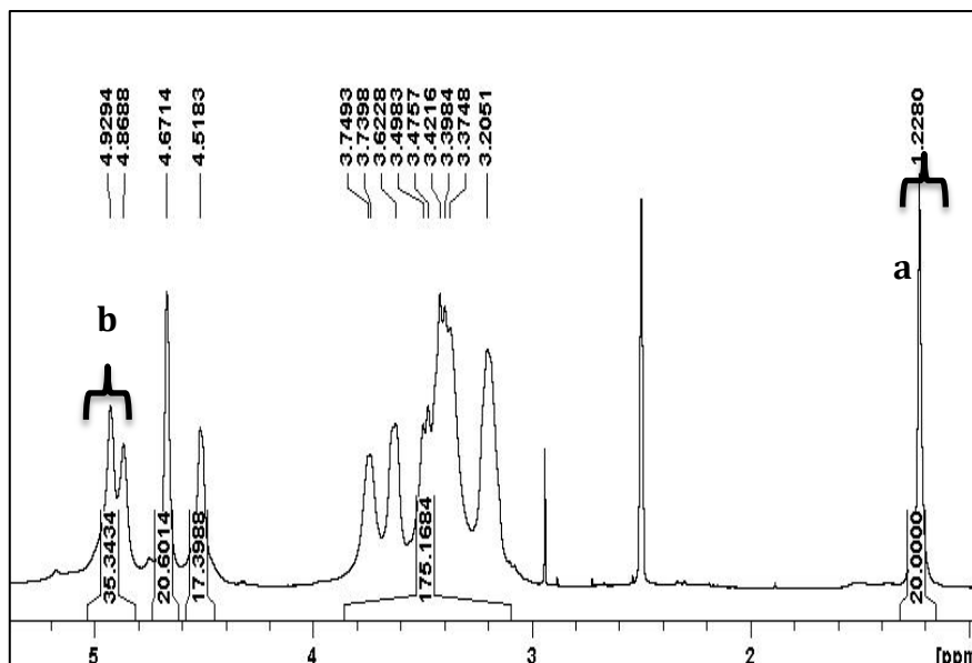
Figure 5-7 1 H-NMR of Dex-DDSA. D.S. is 2.72%.
