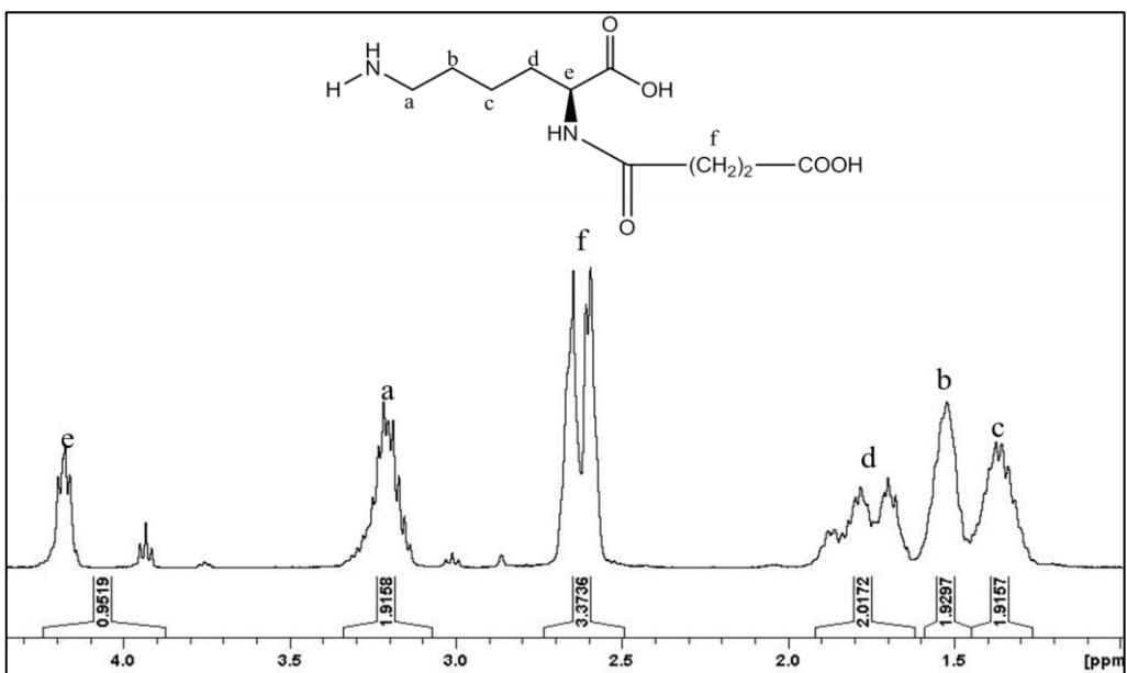
Figure 3-4 1 H NMR of PLL (0.9) Degree of substitution is 85%
