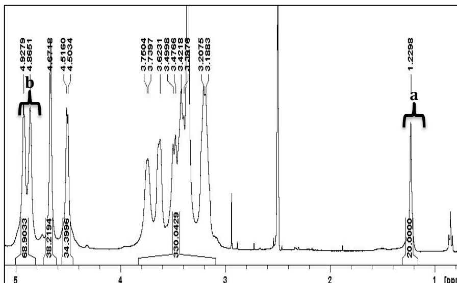
Figure 5-6 1 H-NMR of Dex-DDSA. D.S. is 1.4%
