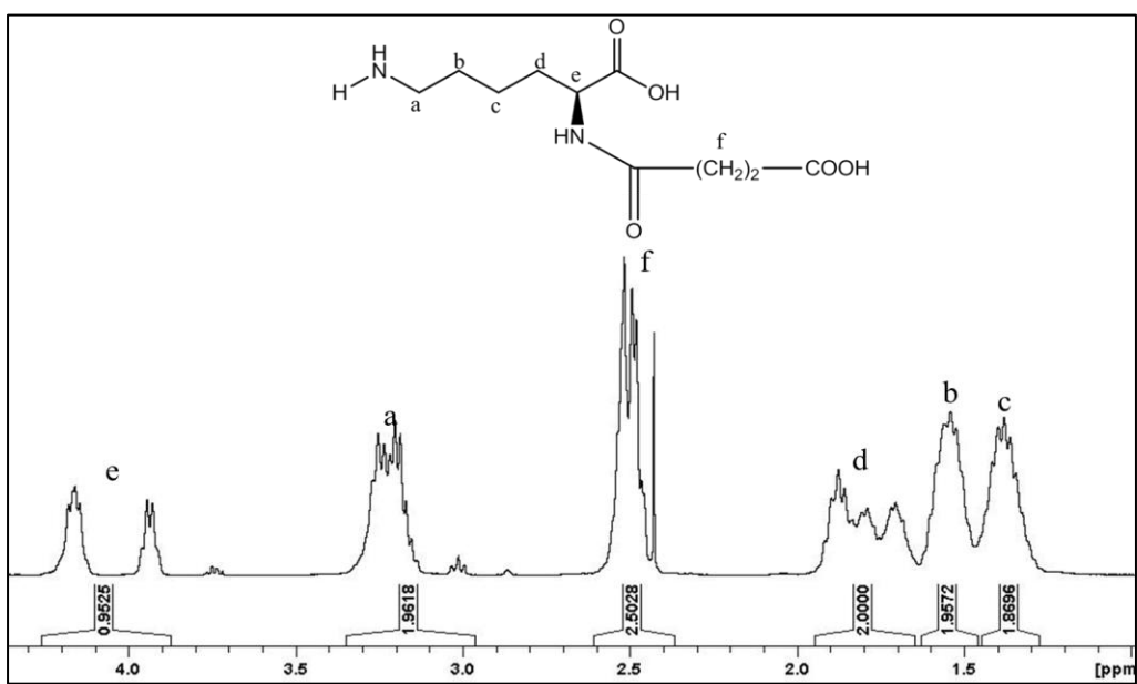
Figure 3-3 1 H NMR of PLL (0.65) Degree of substitution is 63%
