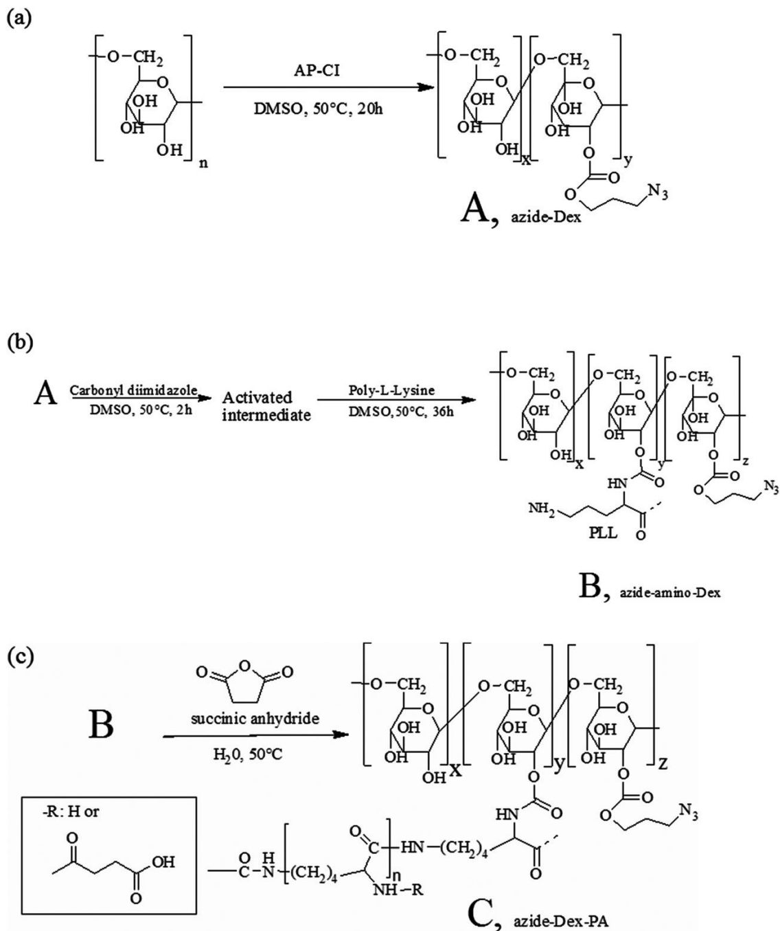
Scheme 1 Schematic representation of the synthesis of dextran polyampholyte (Dex-PA). (a) Substitution of azide in dextran. Dextran and 3-azidopropyl carbonylimidazole reacted to form dextran azopropyl carbonate (azide-Dex, A). (b) Amination of azide-dextran. A was activated with 1,1'-carbonyldiimidazole (CDI), and poly-L-lysine was grafted onto azide-Dex (azide-amino-Dex, B). (c) Succinylation of azide-amino-dextran. Succinic anhydride (SA) reacted with the azide-amino-Dex, yielding the carboxylated azide-amino-Dex (azide-Dex-PA, C).
