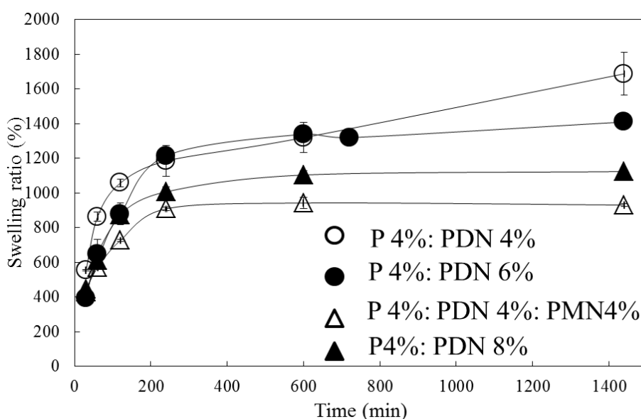
Figure 4-2 Swelling measurements of hydrogels: Swelling ratio is monitored as a function of varying cross-linker concentration. Symbols represent the average for n=3 samples.
