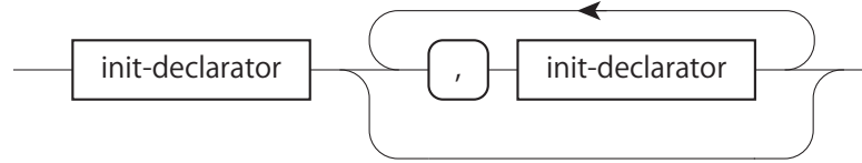
図 A.14: init-declarator-list
