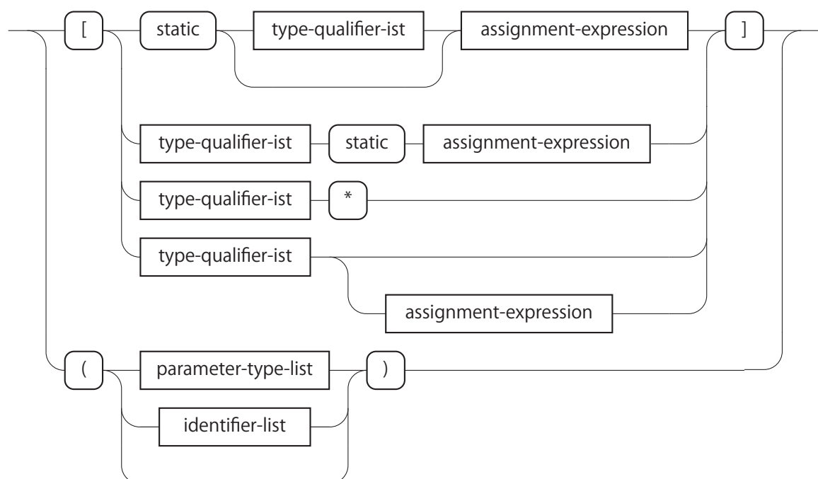
図 A.32: direct-declarator
