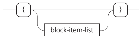
図 A.50: compound-statement
