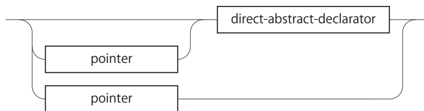
abstract-declarator
