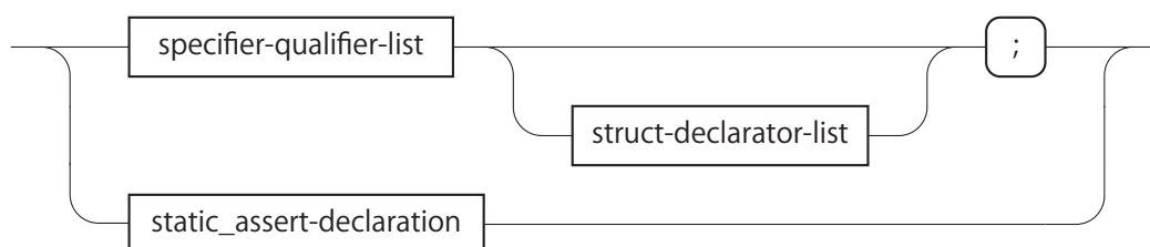
図 A.21: struct-declaration
