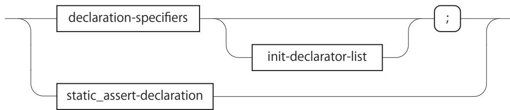
図 A.12: declaration
