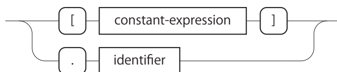
図 A.46: designator
