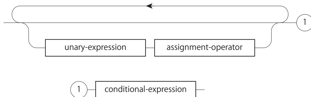
図 A.9: assignment-expression
