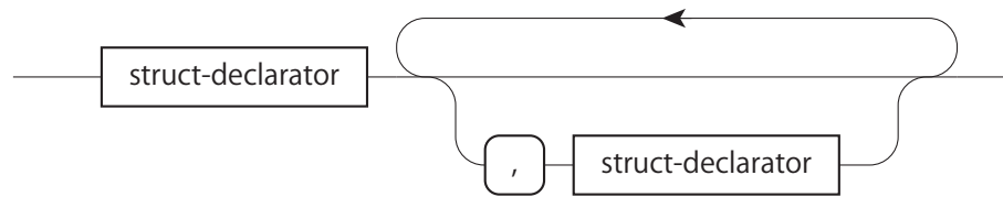
図 A.23: struct-declarator-list
