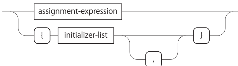
☒ A.42: initializer
