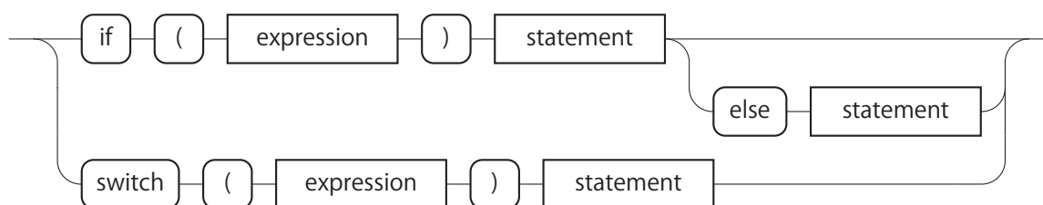
図 A.54: selection-statement
