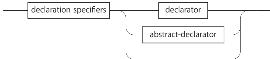
図 A.36: parameter-declaration
