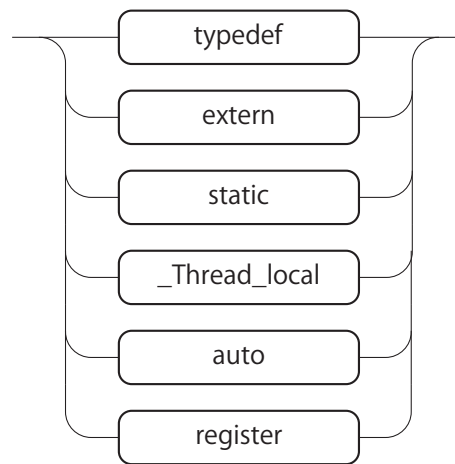
図 A.16: storage-class-specifier
