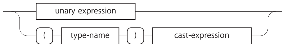
図 A.6: cast-expression
