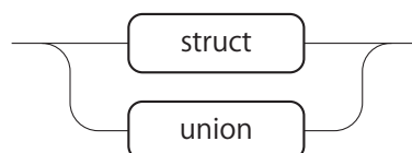
図 A.19: struct-or-union
