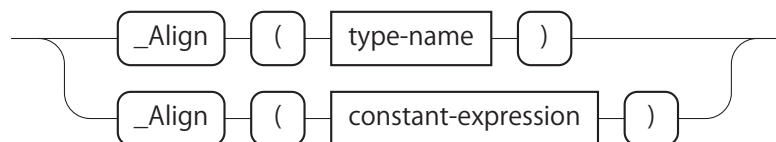
図 A.30: alignment-specifier
