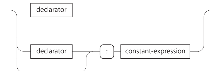
図 A.24: struct-declarator
