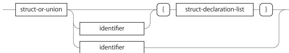
図 A.18: struct-or-union-specifier
