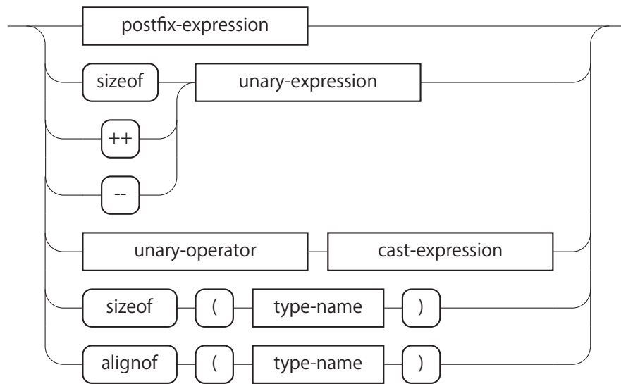
図 A.4: unary-expression
