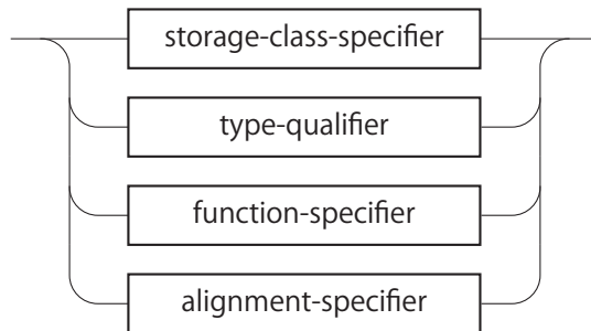
図 A.13: declaration-specifier
