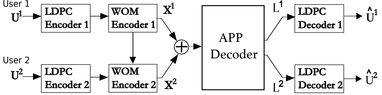
Fig. 6.2 System diagram using LDPC codes.
