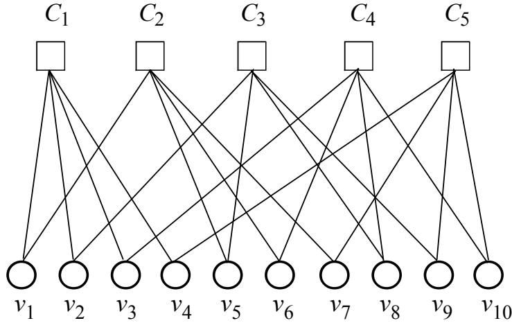
Fig. 6.1 A Tanner graph of the (10, 5) LDPC code.
