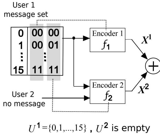
Fig. 8.2 An encoding example achieving a BS-AMAC rate in the bonus region
