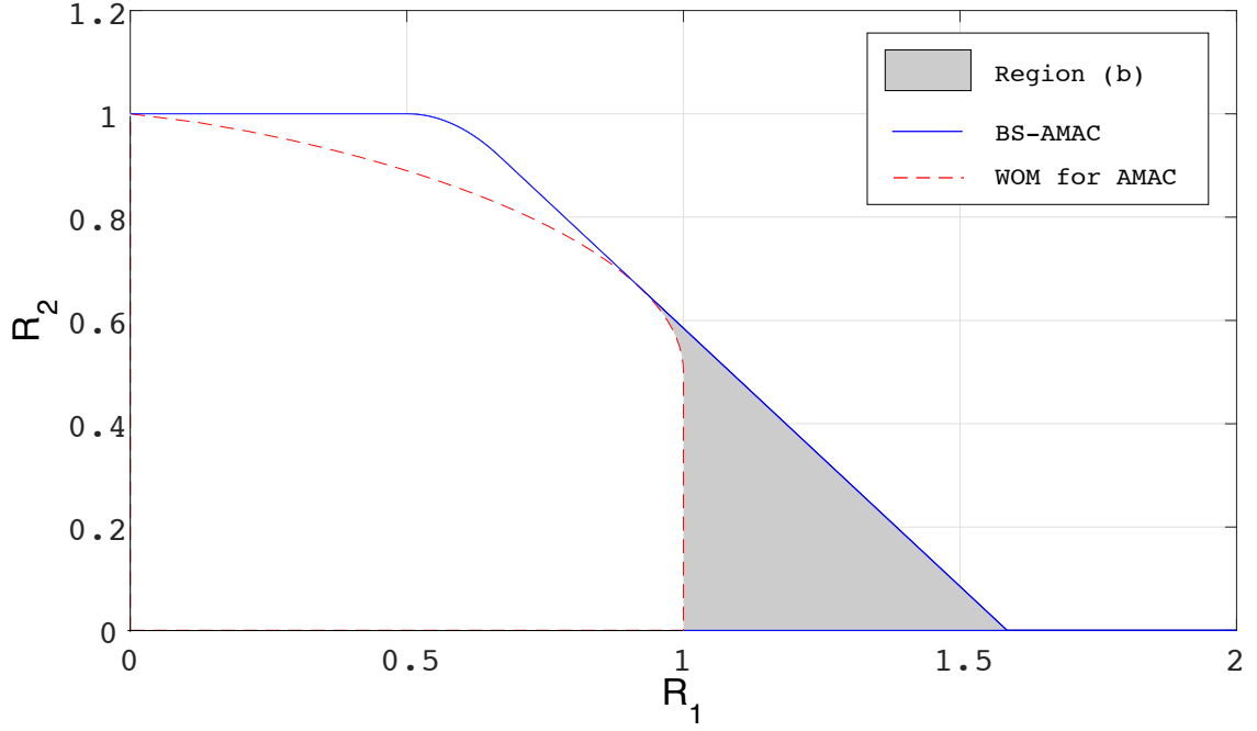
Fig. 8.1 Bonus region (for error free case P_e = 0 ).
