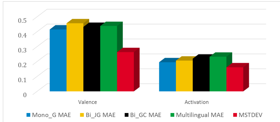
(b) Comparison of MAE and MSTDEV for each Emotion Dimension (ED) in German database.
