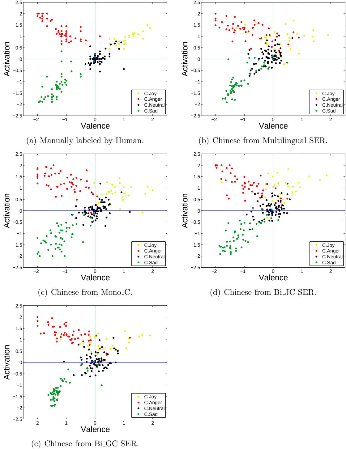
Figure 4.14: Scatter Plot of Estimated Positions of Chinese database in V-A space.
