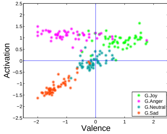
(c) German from Mono_G.
