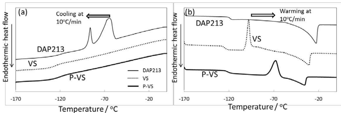
Fig. 1. DSC thermograms of various VSs for (a) cooling and (b) heating at 10^{\circ}\text{C}/\text{min} .
