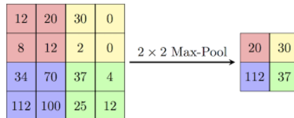
FIGURE 2.8: A max pool example with window size 2x2, stride length 2
