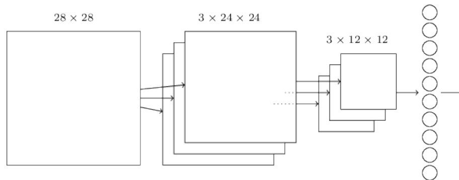
FIGURE 2.9: A complete CNN, take an image of digit number size 28x28 as an input, use 3 filters size 5x5 stride length 1, follow by one max-pooling layer and one fully-connected layer [1]
