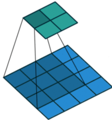
FIGURE 2.7: A window size 3x3, stride length 1, sliding through input grid (blue grid) and connect to next feature map (green grid) [2]
