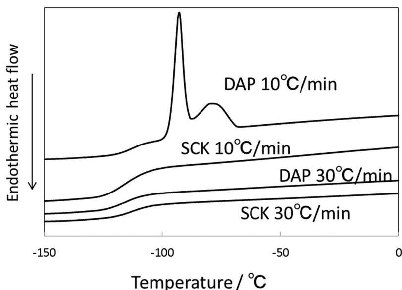
Figure 1. Differential scanning calorimetry (DSC) thermograms of propylene glycol (DAP) and StemCell Keep™ (SCK) for cooling at 10°C/min and 30°C/min.
