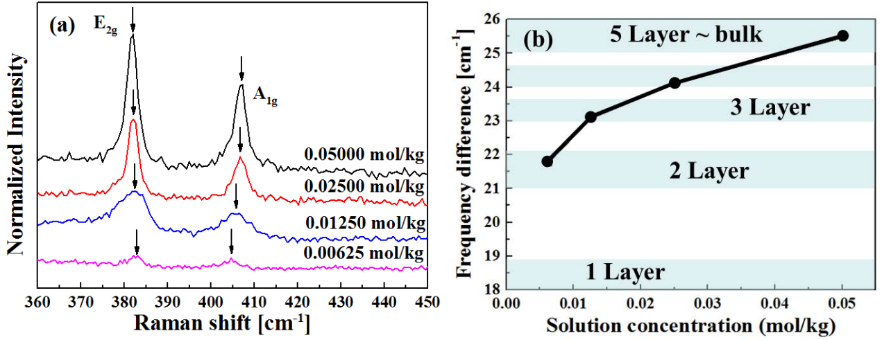
Figure 1. (a) Raman spectra of \text{MoS}_2 fabricated by source solutions with various concentrations. (b) Frequency difference between the peak of the E_{2g} and A_{1g} mode as a function of the concentration of the source solution.
