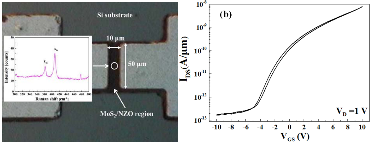
Figure 2(a) Plan view of metal pad for multilayer \text{MoS}_2 transistor and its Raman spectra, (b) the characteristic of (a) gate-voltage and drain current.
