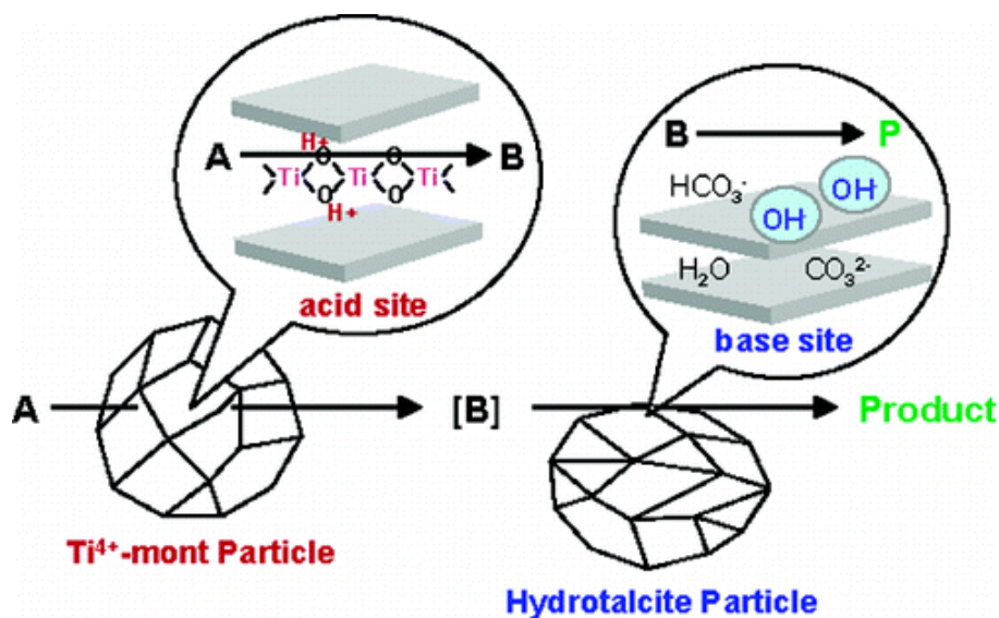
Figure 2 One-pot reaction using acidic Ti 4+ -exchanged motmorillonite and basic hydrotalcite. 13
