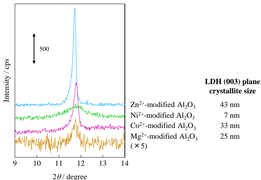
Figure 5 LDH (003) plane XRD peaks of Mg 2+ , Co 2+ , Ni 2+ , and Zn 2+ -modified Al 2 O 3 .
