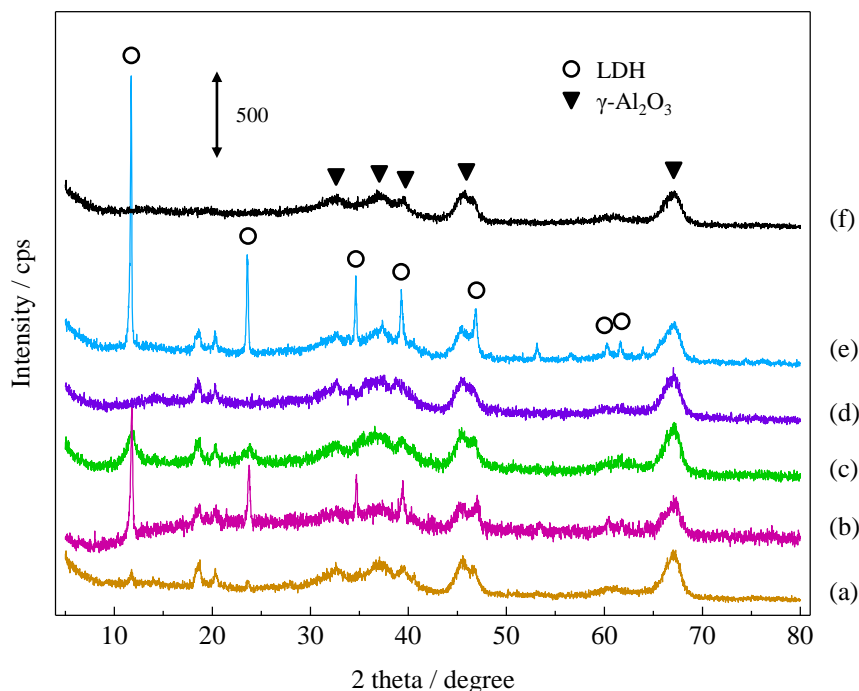
Figure 3 XRD patterns of \gamma -Al 2 O 3 and various M 2+ -modified Al 2 O 3 ; (a) Mg 2+ -modified Al 2 O 3 , (b) Co 2+ -modified Al 2 O 3 , (c) Ni 2+ -modified Al 2 O 3 , (d) Cu 2+ -modified Al 2 O 3 , (e) Zn 2+ -modified Al 2 O 3 and (f) \gamma -Al 2 O 3 .
