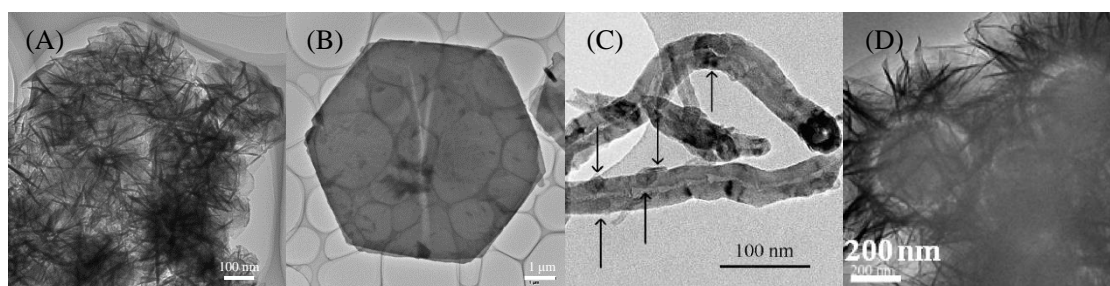
Figure 4 TEM images of LDHs prepared by various methods. (A) co-precipitation, (B) urea co-precipitation, (C) hydrotalcite/carbon 48 and (D) SiO 2 @LDH core-shell. 51
