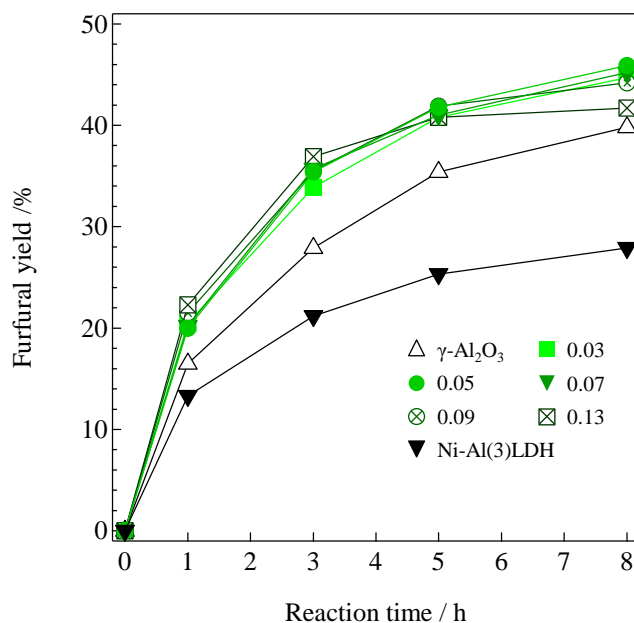
Figure 9 Time cause of one-pot synthesis of furfural from xylose over combined use of Amberlyst-15 and Ni 2+ -modified Al 2 O 3 with various Ni/Al atomic ratio. Reaction conditions: xylose (0.67 mmol), Ni 2+ -modified Al 2 O 3 (0.2 g), Amberlyst-15 (0.1 g), DMF (3 mL), 373 K, N 2 flow (30 mL·min -1 ).
