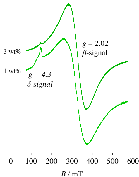
Figure 16 (A) ESR spectra of Cr/Mg-Al LDHs with various Cr loadings and (B) normalized spectra for 1 wt% and 3 wt% at 103 K.
