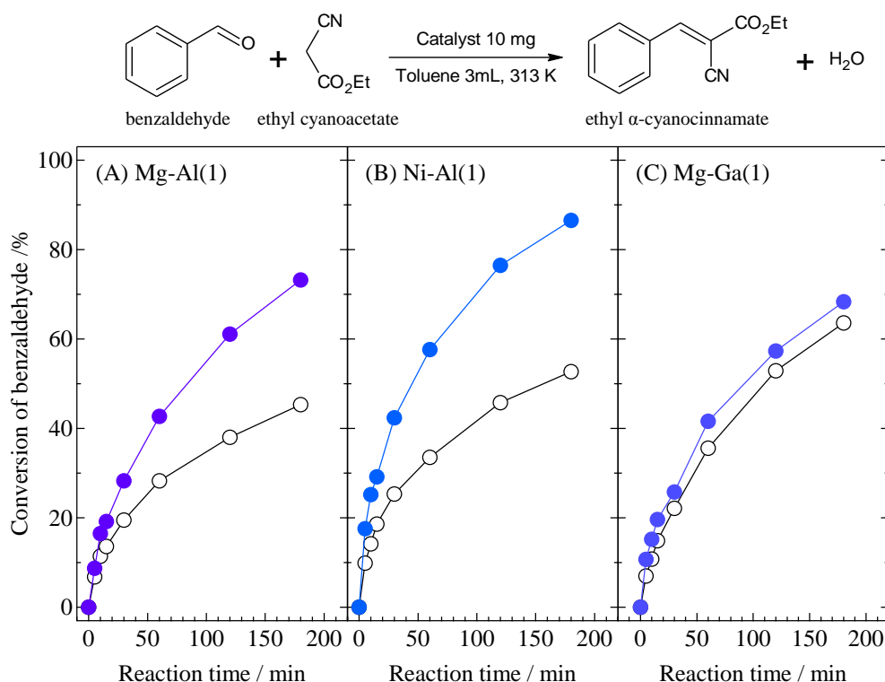
Figure 6 Activities of (○) M^{2+} - M^{3+} (1)LDH and (●) SiO 2 (40nm)@ M^{2+} - M^{3+} (1)LDH with various metal compositions for the Knoevenagel condensation of benzaldehyde with ethyl cyanoacetate. Reaction conditions: benzaldehyde (0.5 mmol), ethyl cyanoacetate (0.6 mmol), catalyst (10 mg), toluene (3 mL), 313 K, N 2 flow (30 mL min -1 ).
