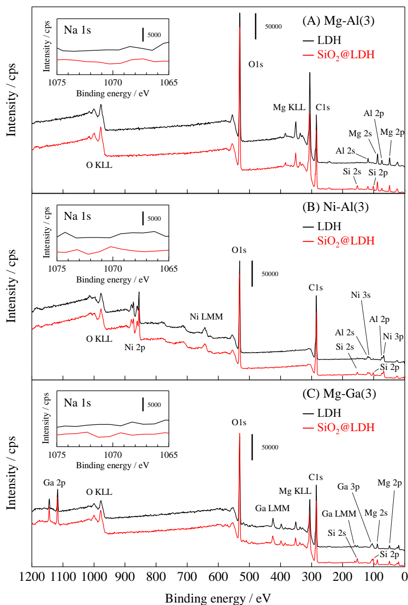
Figure 3 Survey XPS spectra of \text{M}^{2+}\text{-M}^{3+}(3)\text{LDHs} and \text{SiO}_2(40\text{nm})@\text{M}^{2+}\text{-M}^{3+}(3)\text{LDHs} .
