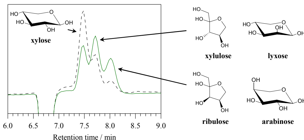
Figure 2 HPLC chart of transformation of xylose using Mg-Al LDH (dashed line) and 9wt%Cr/Mg-Al LDH (solid line). Reaction conditions: xylose (0.67 mmol), catalyst (0.2 g), N,N -dimethylformamide (3 mL), 373 K, 3 h, 500 rpm, and \text{N}_2 flow (30 mL min -1 ).
