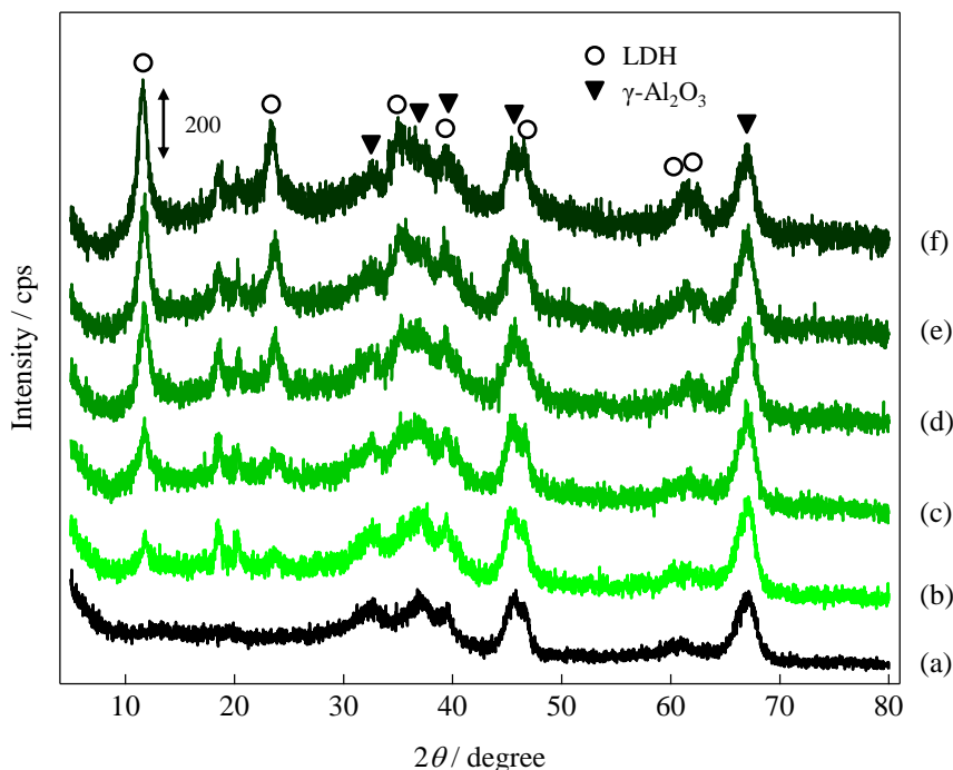
Figure 8 XRD patterns of (a) \gamma -Al 2 O 3 and Ni 2+ -modified Al 2 O 3 with various Ni/Al atomic ratio of (b) 0.03, (c) 0.05, (d) 0.07, (e) 0.09 and (f) 0.13.
