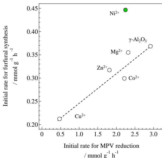
Figure 4 Correlation of activities for MPV reduction and furfural synthesis over various M 2+ -modified Al 2 O 3 catalysts.
