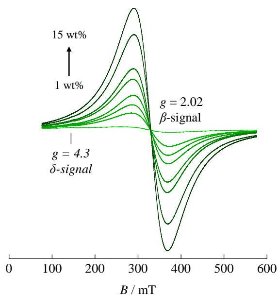
Figure 16 (A) ESR spectra of Cr/Mg-Al LDHs with various Cr loadings and (B) normalized spectra for 1 wt% and 3 wt% at 103 K.
