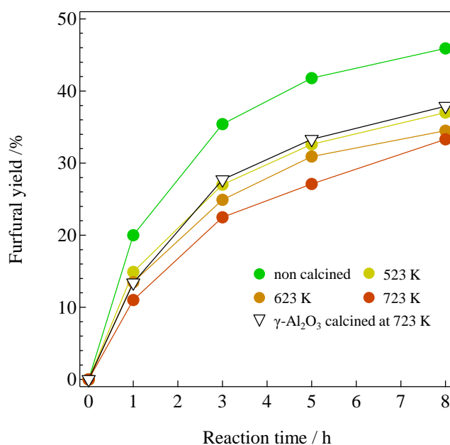
Figure 11 Time course of one-pot synthesis of furfural from xylose over combined use of Amberlyst-15 and calcined Ni 2+ -modified Al 2 O 3 at various temperature. Reaction conditions: xylose (0.67 mmol), Ni 2+ -modified Al 2 O 3 (0.2 g), Amberlyst-15 (0.1 g), DMF (3 mL), 373 K, N 2 flow (30 mL·min -1 ).
