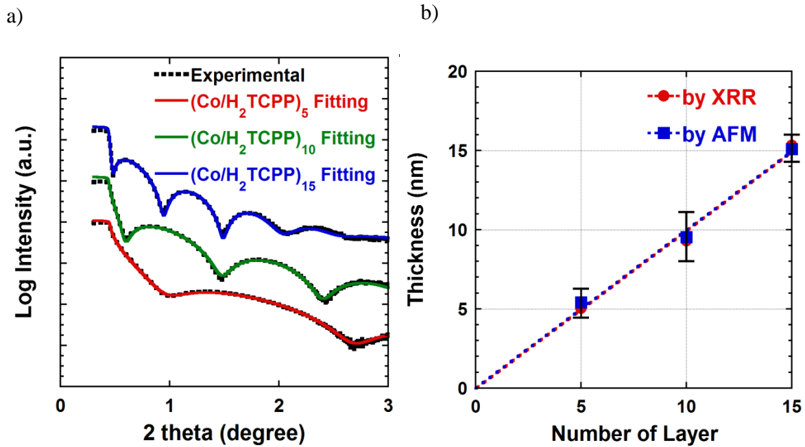
Figure 2. (a) XRR profiles of multilayer films (Co/H 2 TCPP) 5 , (Co/H 2 TCPP) 10 , and (Co/H 2 TCPP) 15 on the APTMS-modified Si-wafer substrates. Experimental and fitted data are shown respectively as dashed line and solid line. (b) Thickness of multilayer film comparing between XRR and AFM study with the error bar.
