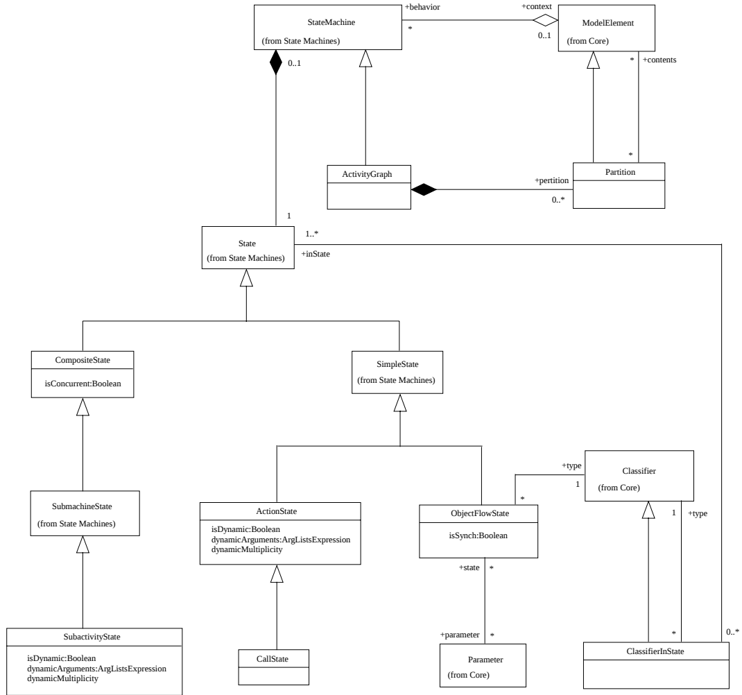
図 5.15: Activity Graphs
