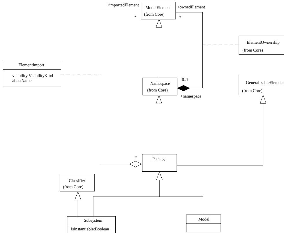
図 5.16: Model Management
