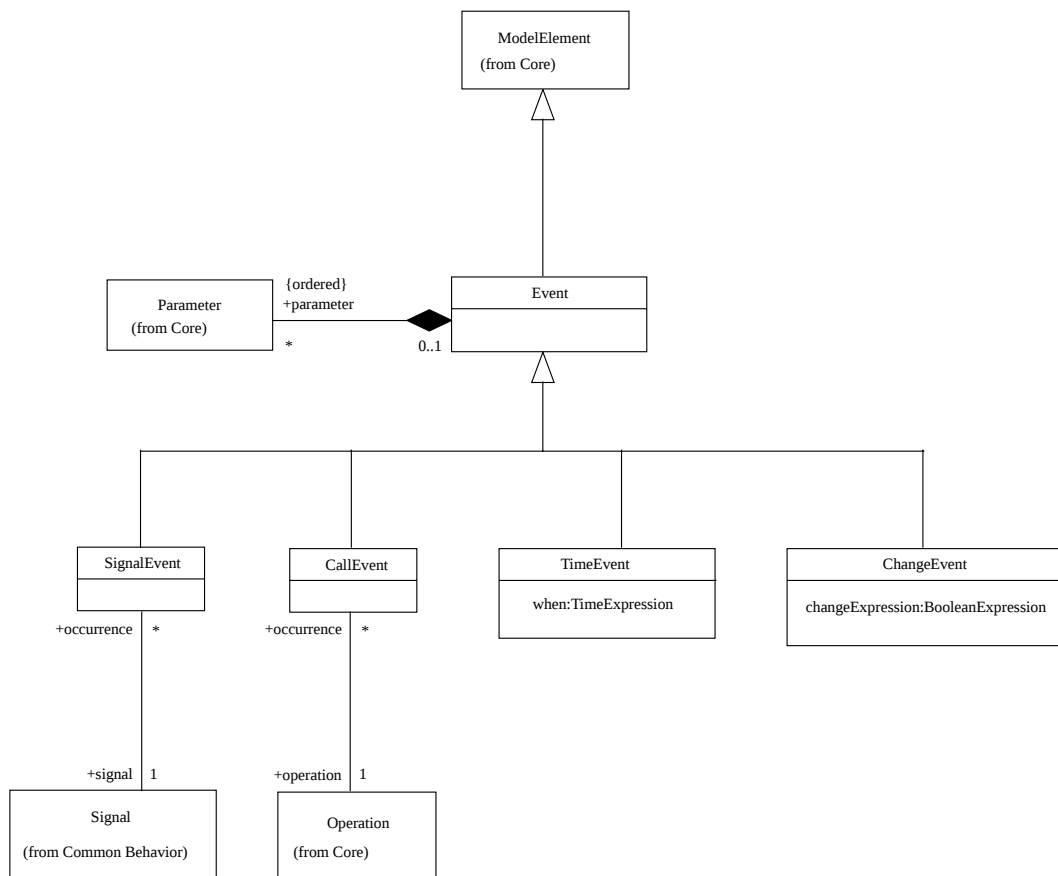
図 5.14: State Machines - Events
