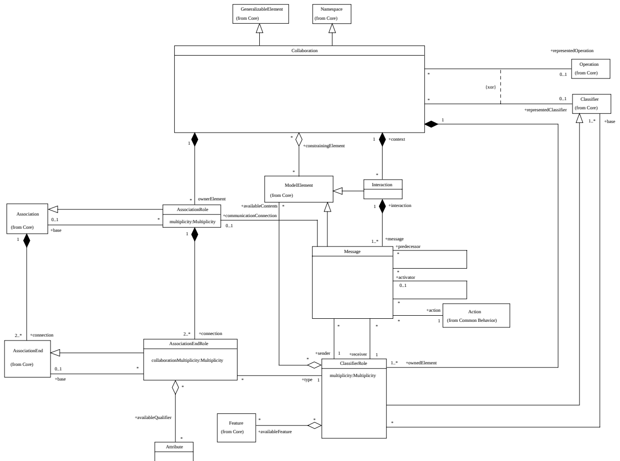
図 5.11: Collaborations
