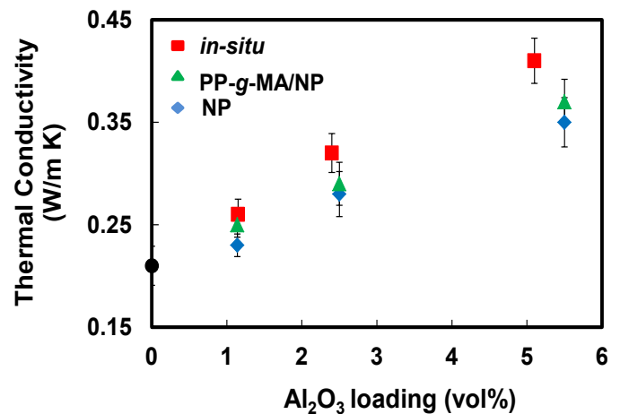
Fig. 3. Thermal conductivity of PP/Al 2 O 3 nanocomposites.
