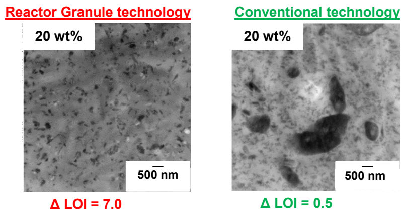
Fig. 1. Results for PP/Mg(OH) 2 nanocomposites.
