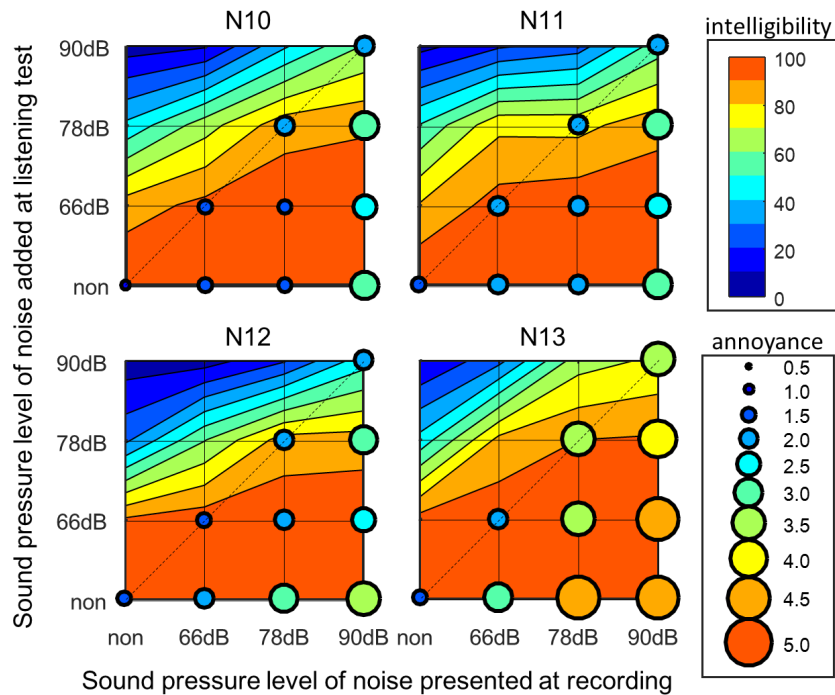
Figure 3: Estimated intelligibility (contour plot), and annoyance rating (bubble chart) by speaker.
